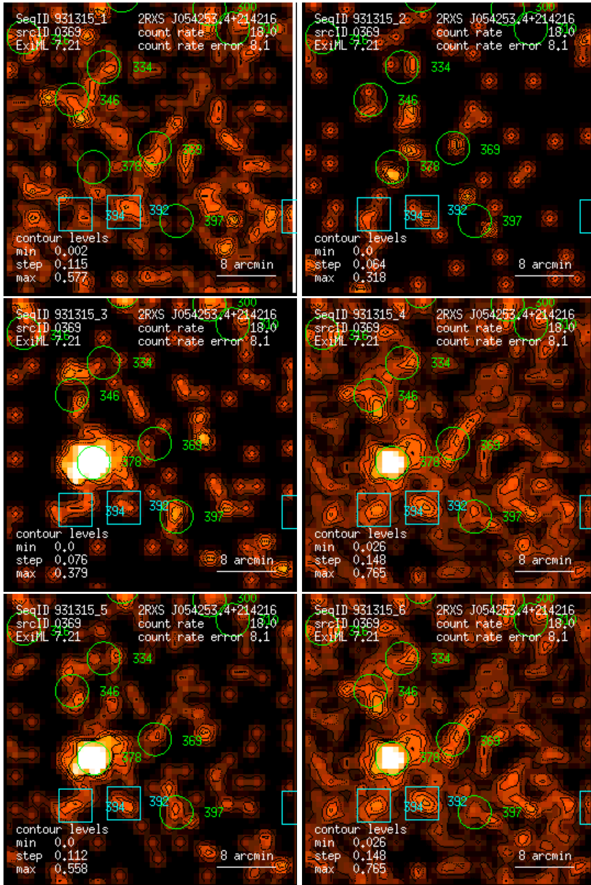
Figure 369: RASS 931315: detection 0369: band rate images, Gaussian filter: (1) PSPC channels 11 – 41, (2) 52 – 90, (3) 91 – 201, (4) 11 – 235, (5) 52 – 201, (6) 11 – 201. Broad band rates in counts/ks. Band rate contour levels in counts/ks/arcmin 2 .
