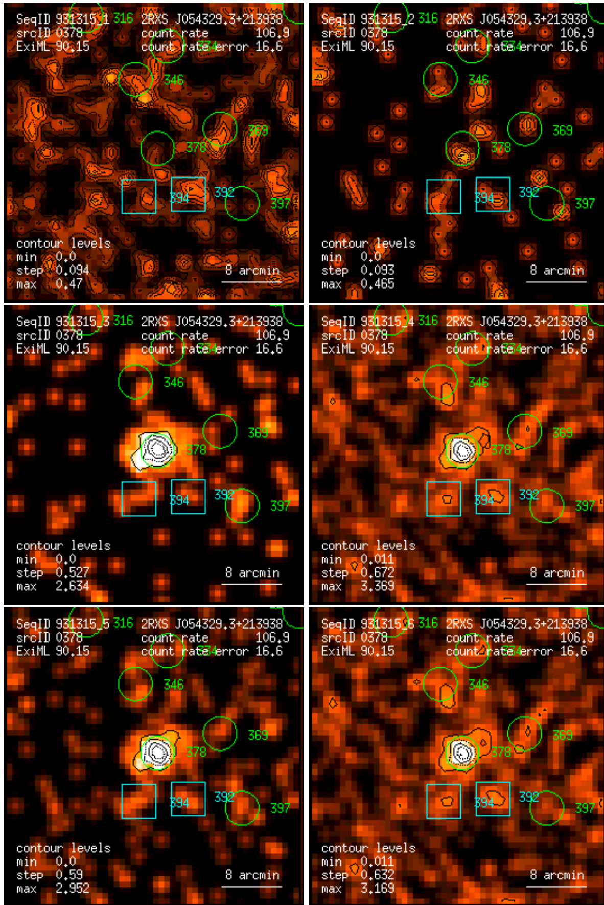
Figure 378: RASS 931315: detection 0378: band rate images, Gaussian filter: (1) PSPC channels 11 – 41, (2) 52 – 90, (3) 91 – 201, (4) 11 – 235, (5) 52 – 201, (6) 11 – 201. Broad band rates in counts/ks. Band rate contour levels in counts/ks/arcmin 2 .
