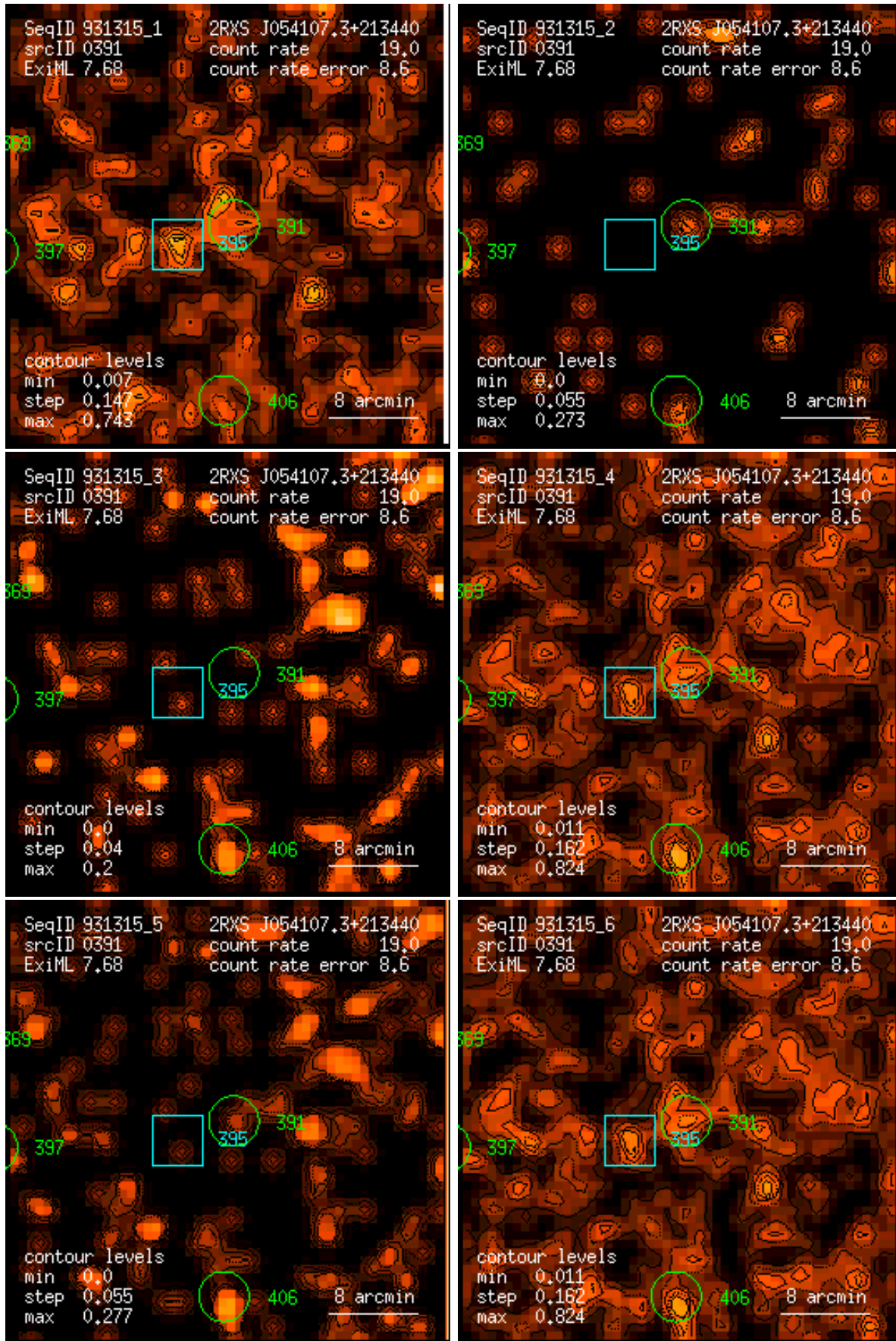
Figure 391: RASS 931315: detection 0391: band rate images, Gaussian filter: (1) PSPC channels 11 – 41, (2) 52 – 90, (3) 91 – 201, (4) 11 – 235, (5) 52 – 201, (6) 11 – 201. Broad band rates in counts/ks. Band rate contour levels in counts/ks/arcmin 2 .
