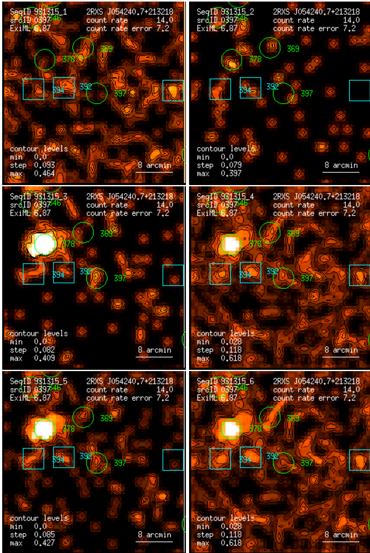
Figure 397: RASS 931315: detection 0397: band rate images, Gaussian filter: (1) PSPC channels 11 – 41, (2) 52 – 90, (3) 91 – 201, (4) 11 – 235, (5) 52 – 201, (6) 11 – 201. Broad band rates in counts/ks. Band rate contour levels in counts/ks/arcmin 2 .
