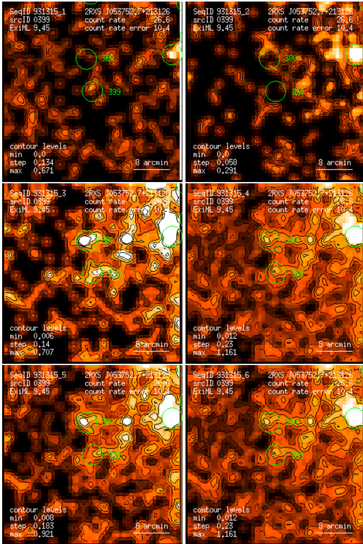
Figure 399: RASS 931315: detection 0399: band rate images, Gaussian filter: (1) PSPC channels 11 – 41, (2) 52 – 90, (3) 91 – 201, (4) 11 – 235, (5) 52 – 201, (6) 11 – 201. Broad band rates in counts/ks. Band rate contour levels in counts/ks/arcmin 2 .
