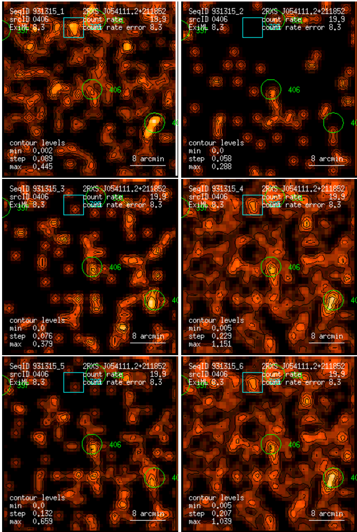
Figure 406: RASS 931315: detection 0406: band rate images, Gaussian filter: (1) PSPC channels 11 – 41, (2) 52 – 90, (3) 91 – 201, (4) 11 – 235, (5) 52 – 201, (6) 11 – 201. Broad band rates in counts/ks. Band rate contour levels in counts/ks/arcmin 2 .
