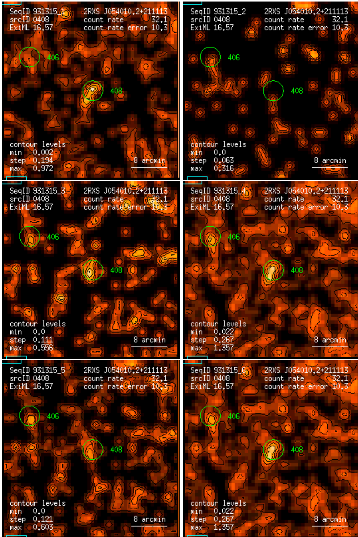
Figure 408: RASS 931315: detection 0408: band rate images, Gaussian filter: (1) PSPC channels 11 – 41, (2) 52 – 90, (3) 91 – 201, (4) 11 – 235, (5) 52 – 201, (6) 11 – 201. Broad band rates in counts/ks. Band rate contour levels in counts/ks/arcmin 2 .
