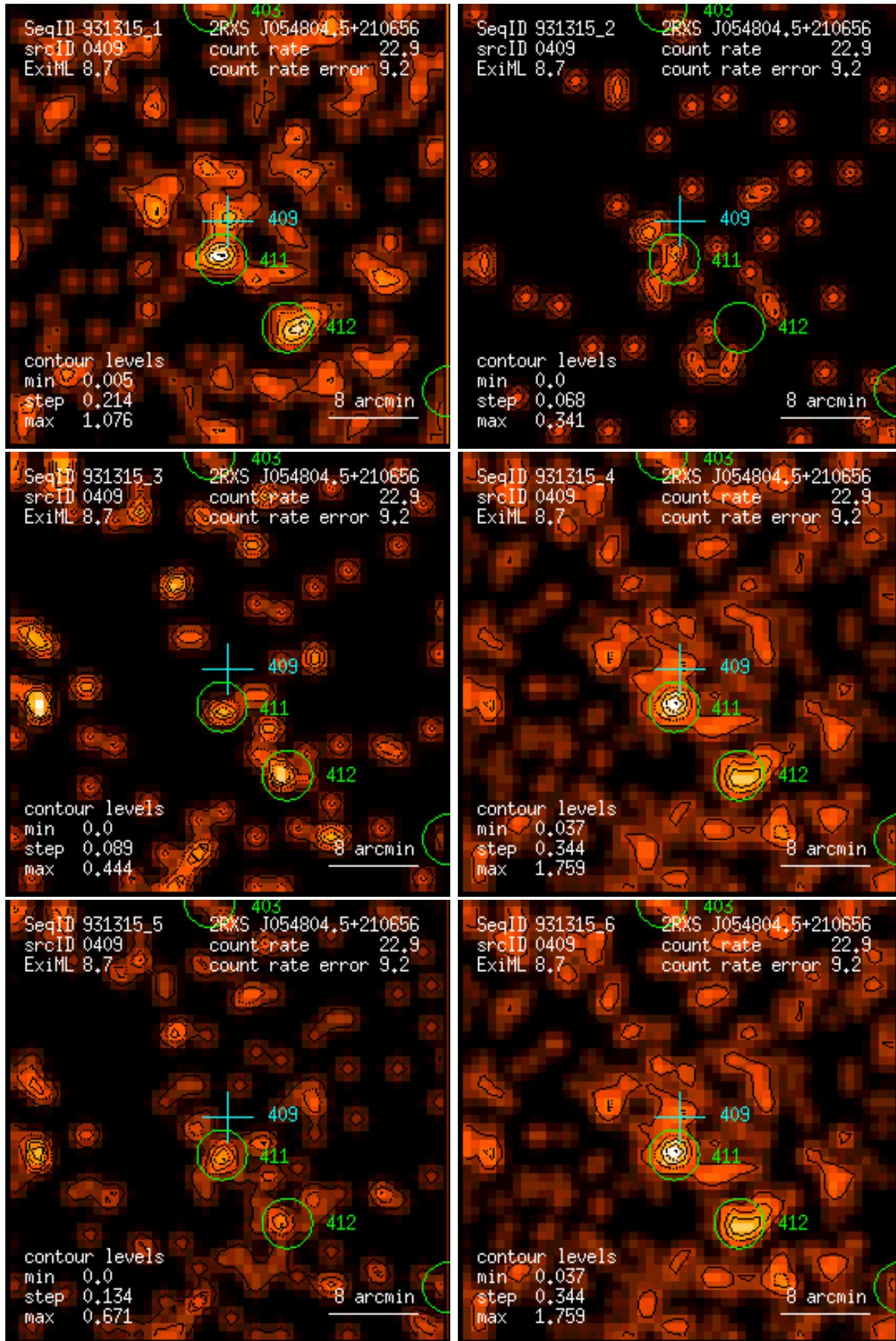
Figure 409: RASS 931315: detection 0409: band rate images, Gaussian filter: (1) PSPC channels 11 – 41, (2) 52 – 90, (3) 91 – 201, (4) 11 – 235, (5) 52 – 201, (6) 11 – 201. Broad band rates in counts/ks. Band rate contour levels in counts/ks/arcmin 2 .
