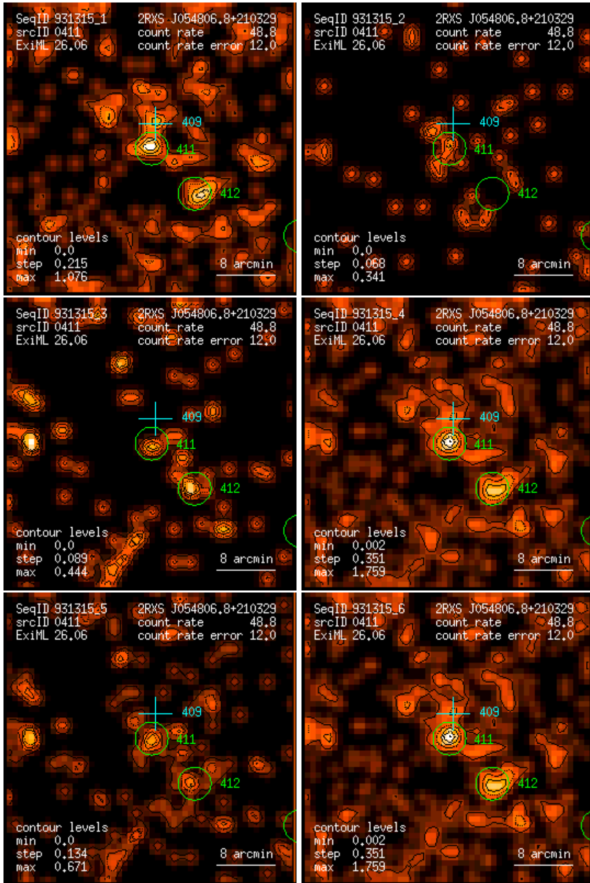
Figure 411: RASS 931315: detection 0411: band rate images, Gaussian filter: (1) PSPC channels 11 – 41, (2) 52 – 90, (3) 91 – 201, (4) 11 – 235, (5) 52 – 201, (6) 11 – 201. Broad band rates in counts/ks. Band rate contour levels in counts/ks/arcmin 2 .
