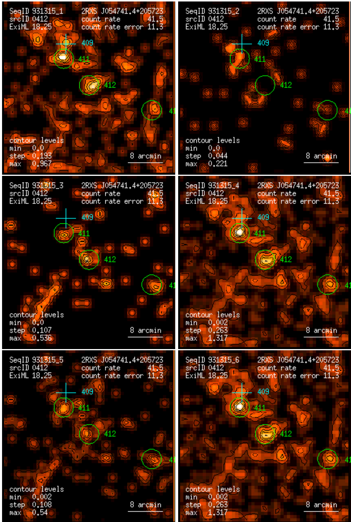
Figure 412: RASS 931315: detection 0412: band rate images, Gaussian filter: (1) PSPC channels 11 – 41, (2) 52 – 90, (3) 91 – 201, (4) 11 – 235, (5) 52 – 201, (6) 11 – 201. Broad band rates in counts/ks. Band rate contour levels in counts/ks/arcmin 2 .
