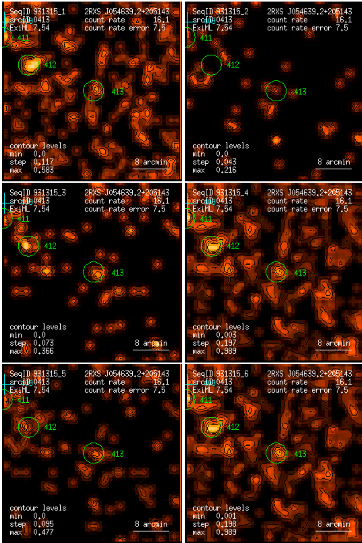
Figure 413: RASS 931315: detection 0413: band rate images, Gaussian filter: (1) PSPC channels 11 – 41, (2) 52 – 90, (3) 91 – 201, (4) 11 – 235, (5) 52 – 201, (6) 11 – 201. Broad band rates in counts/ks. Band rate contour levels in counts/ks/arcmin 2 .
