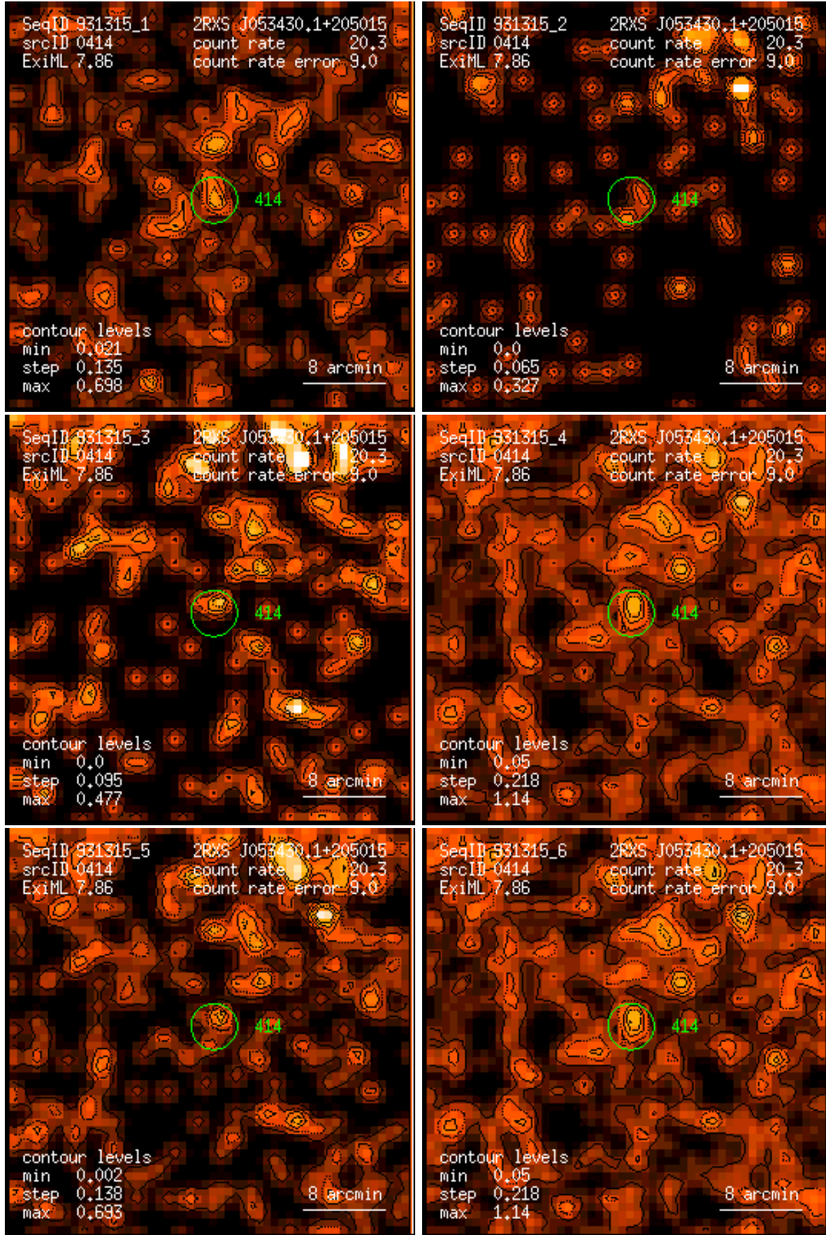
Figure 414: RASS 931315: detection 0414: band rate images, Gaussian filter: (1) PSPC channels 11 – 41, (2) 52 – 90, (3) 91 – 201, (4) 11 – 235, (5) 52 – 201, (6) 11 – 201. Broad band rates in counts/ks. Band rate contour levels in counts/ks/arcmin 2 .
