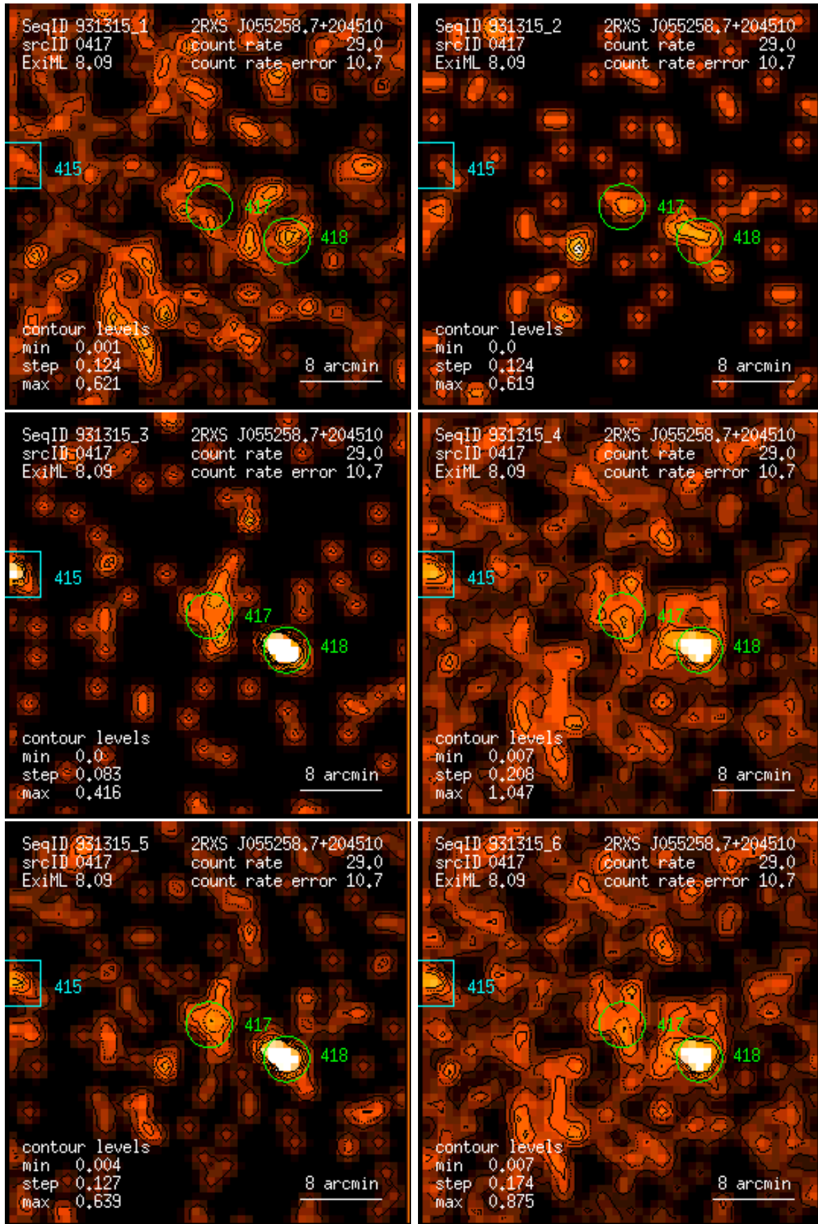
Figure 417: RASS 931315: detection 0417: band rate images, Gaussian filter: (1) PSPC channels 11 – 41, (2) 52 – 90, (3) 91 – 201, (4) 11 – 235, (5) 52 – 201, (6) 11 – 201. Broad band rates in counts/ks. Band rate contour levels in counts/ks/arcmin 2 .
