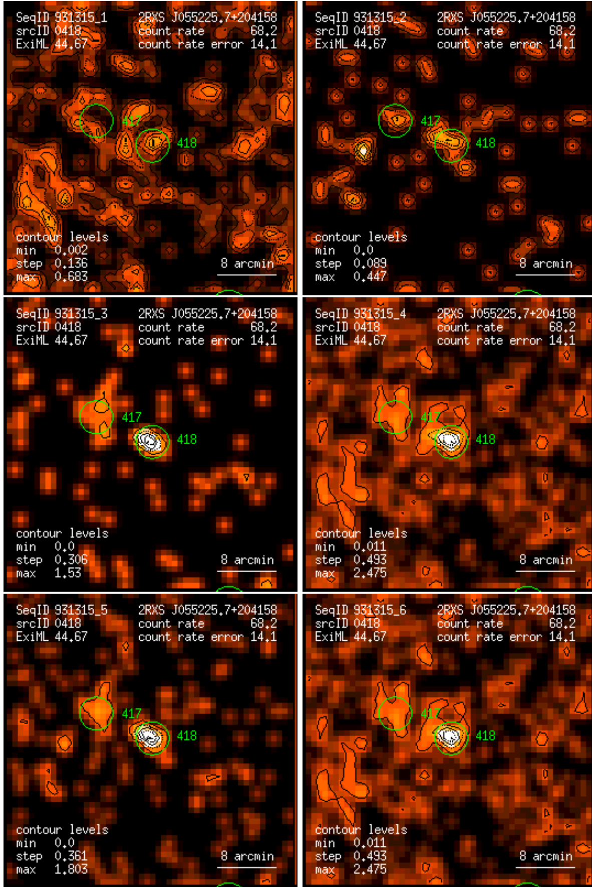
Figure 418: RASS 931315: detection 0418: band rate images, Gaussian filter: (1) PSPC channels 11 – 41, (2) 52 – 90, (3) 91 – 201, (4) 11 – 235, (5) 52 – 201, (6) 11 – 201. Broad band rates in counts/ks. Band rate contour levels in counts/ks/arcmin 2 .
