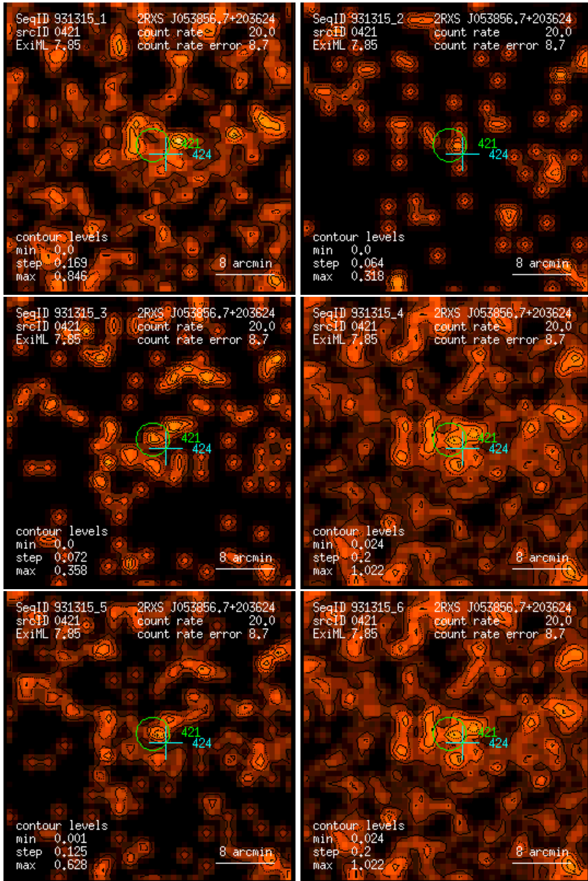
Figure 421: RASS 931315: detection 0421: band rate images, Gaussian filter: (1) PSPC channels 11 – 41, (2) 52 – 90, (3) 91 – 201, (4) 11 – 235, (5) 52 – 201, (6) 11 – 201. Broad band rates in counts/ks. Band rate contour levels in counts/ks/arcmin 2 .
