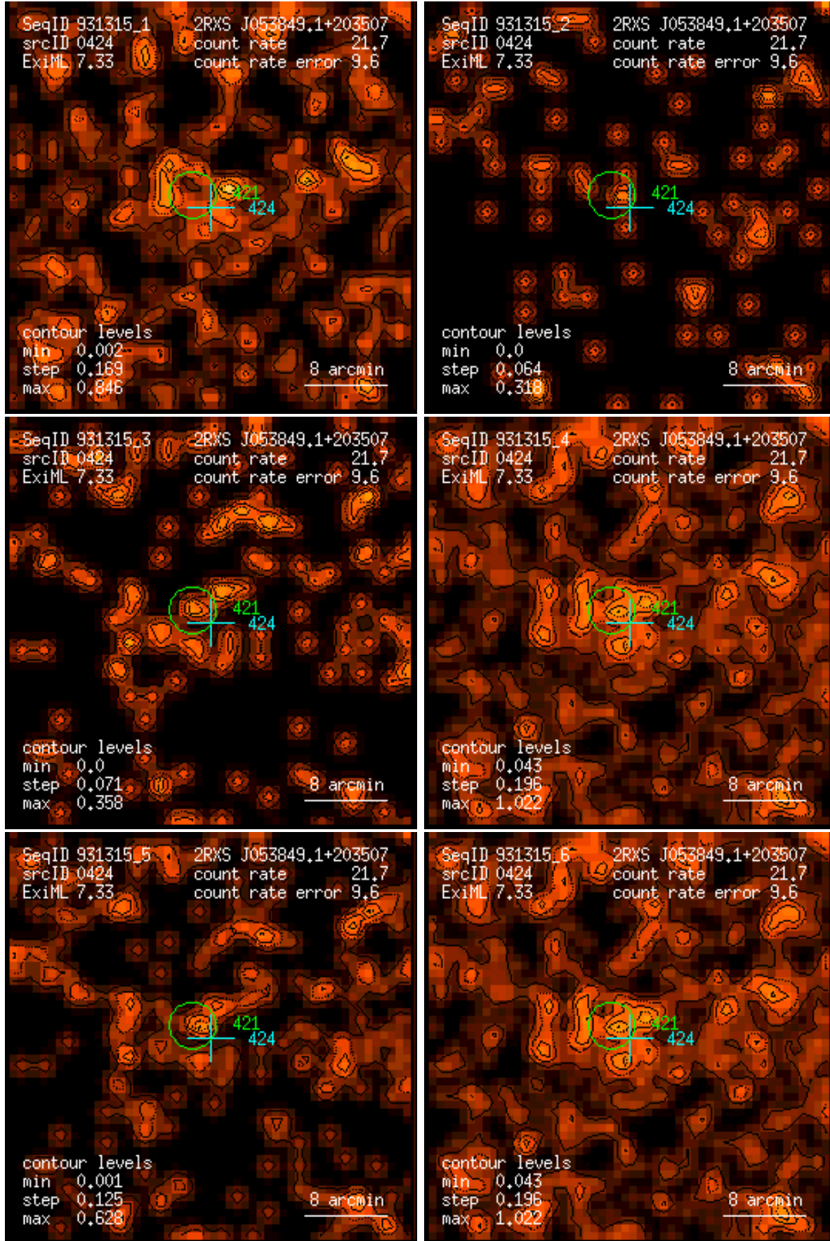
Figure 424: RASS 931315: detection 0424: band rate images, Gaussian filter: (1) PSPC channels 11 – 41, (2) 52 – 90, (3) 91 – 201, (4) 11 – 235, (5) 52 – 201, (6) 11 – 201. Broad band rates in counts/ks. Band rate contour levels in counts/ks/arcmin 2 .
