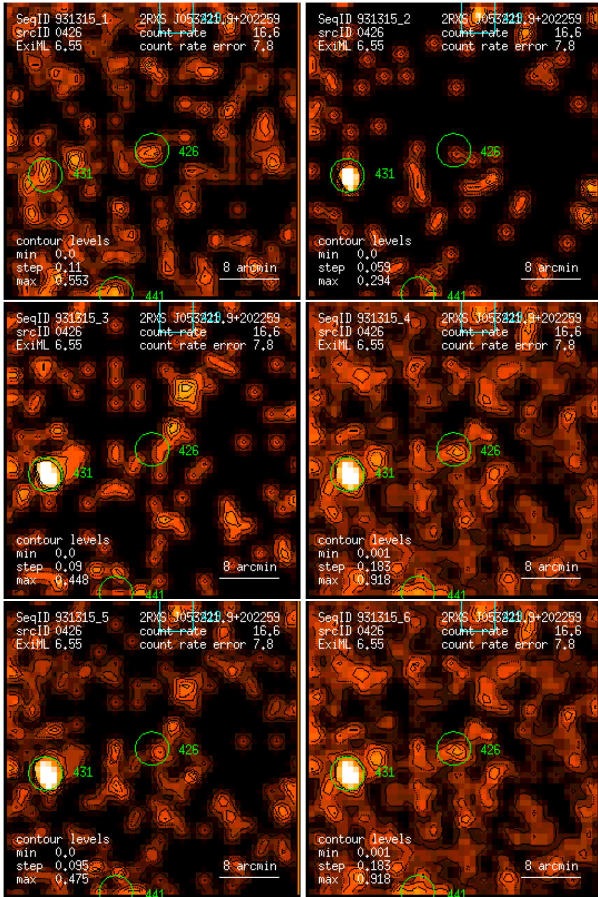
Figure 426: RASS 931315: detection 0426: band rate images, Gaussian filter: (1) PSPC channels 11 – 41, (2) 52 – 90, (3) 91 – 201, (4) 11 – 235, (5) 52 – 201, (6) 11 – 201. Broad band rates in counts/ks. Band rate contour levels in counts/ks/arcmin 2 .
