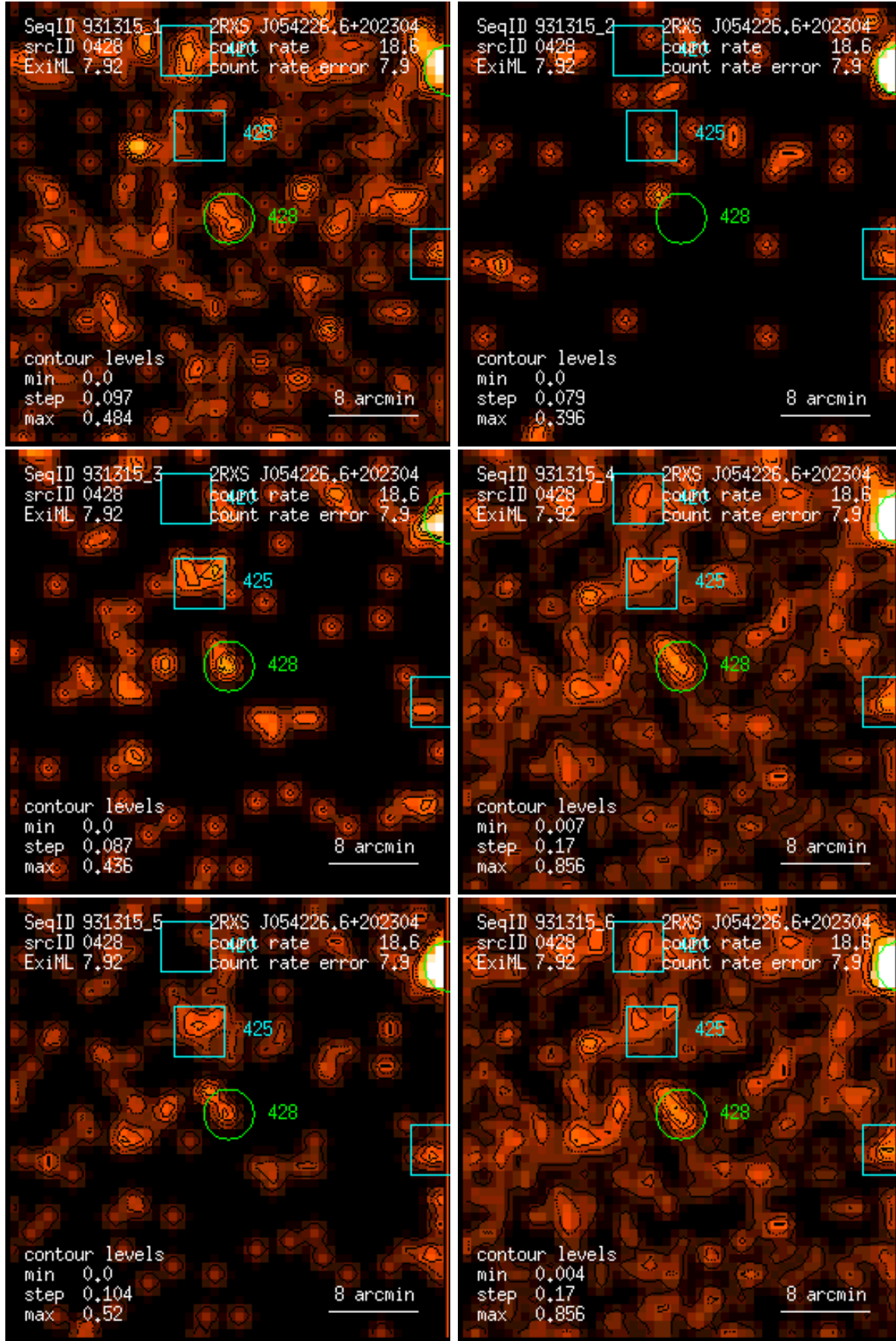
Figure 428: RASS 931315: detection 0428: band rate images, Gaussian filter: (1) PSPC channels 11 – 41, (2) 52 – 90, (3) 91 – 201, (4) 11 – 235, (5) 52 – 201, (6) 11 – 201. Broad band rates in counts/ks. Band rate contour levels in counts/ks/arcmin 2 .
