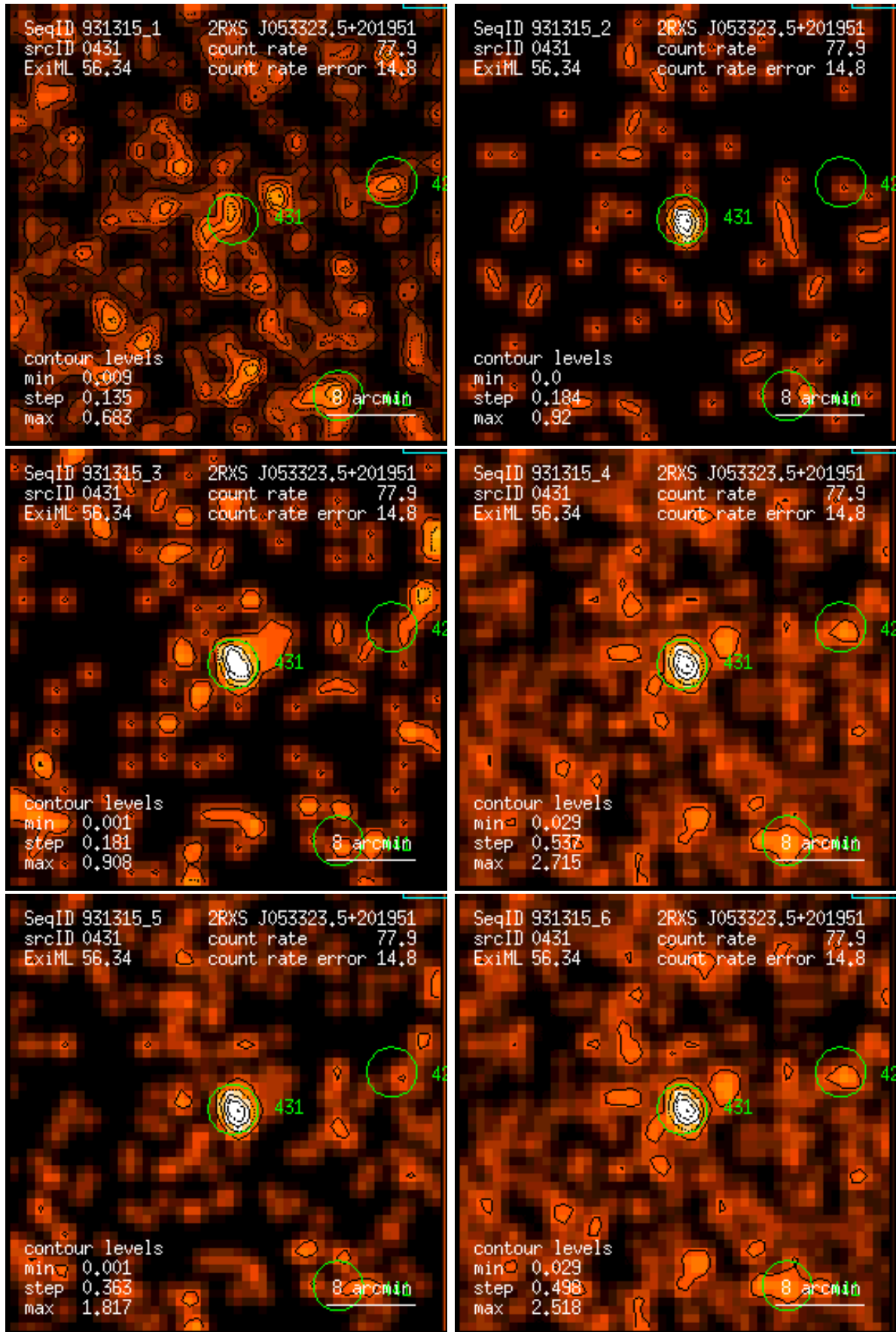
Figure 431: RASS 931315: detection 0431: band rate images, Gaussian filter: (1) PSPC channels 11 – 41, (2) 52 – 90, (3) 91 – 201, (4) 11 – 235, (5) 52 – 201, (6) 11 – 201. Broad band rates in counts/ks. Band rate contour levels in counts/ks/arcmin 2 .
