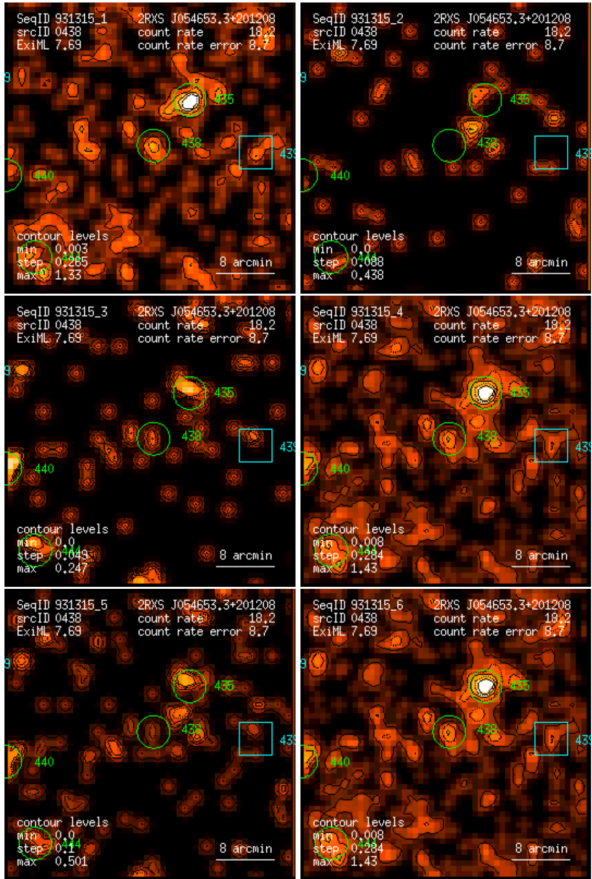
Figure 438: RASS 931315: detection 0438: band rate images, Gaussian filter: (1) PSPC channels 11 – 41, (2) 52 – 90, (3) 91 – 201, (4) 11 – 235, (5) 52 – 201, (6) 11 – 201. Broad band rates in counts/ks. Band rate contour levels in counts/ks/arcmin 2 .
