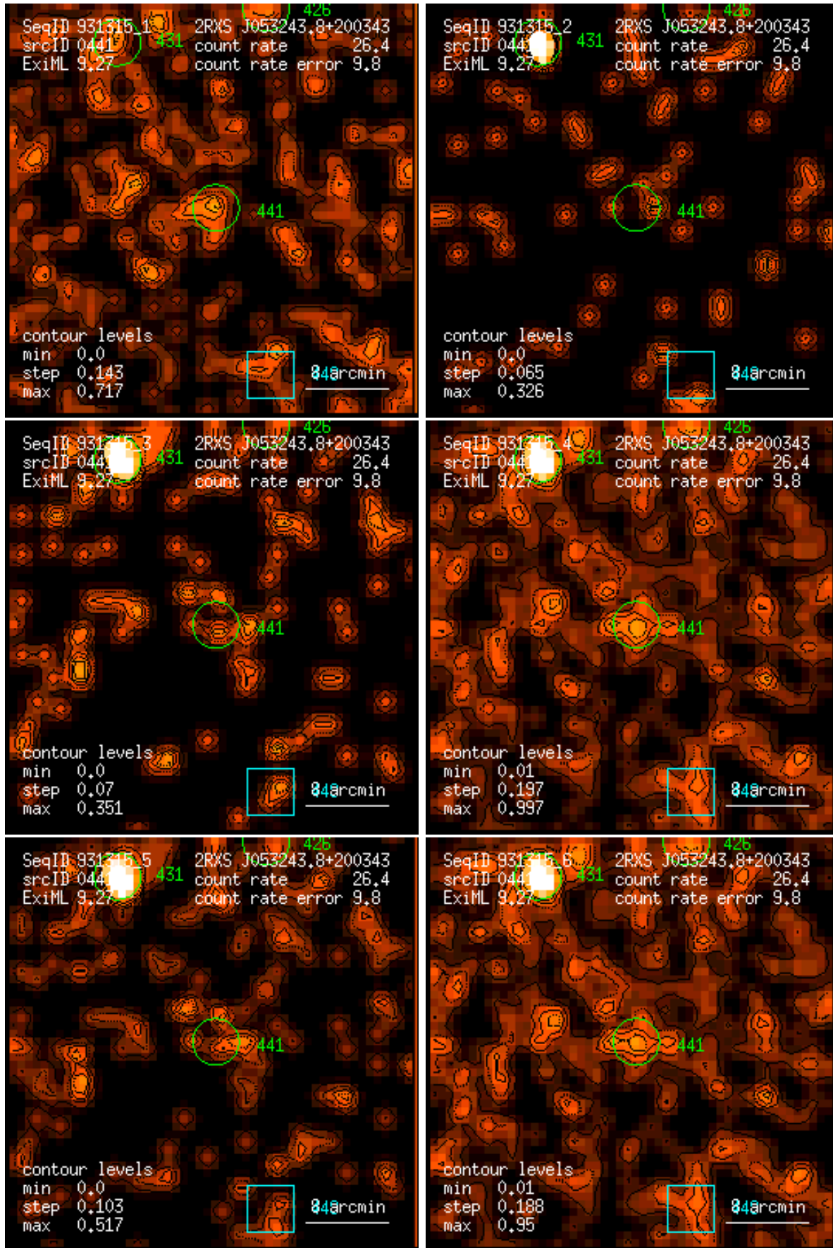
Figure 441: RASS 931315: detection 0441: band rate images, Gaussian filter: (1) PSPC channels 11 – 41, (2) 52 – 90, (3) 91 – 201, (4) 11 – 235, (5) 52 – 201, (6) 11 – 201. Broad band rates in counts/ks. Band rate contour levels in counts/ks/arcmin 2 .
