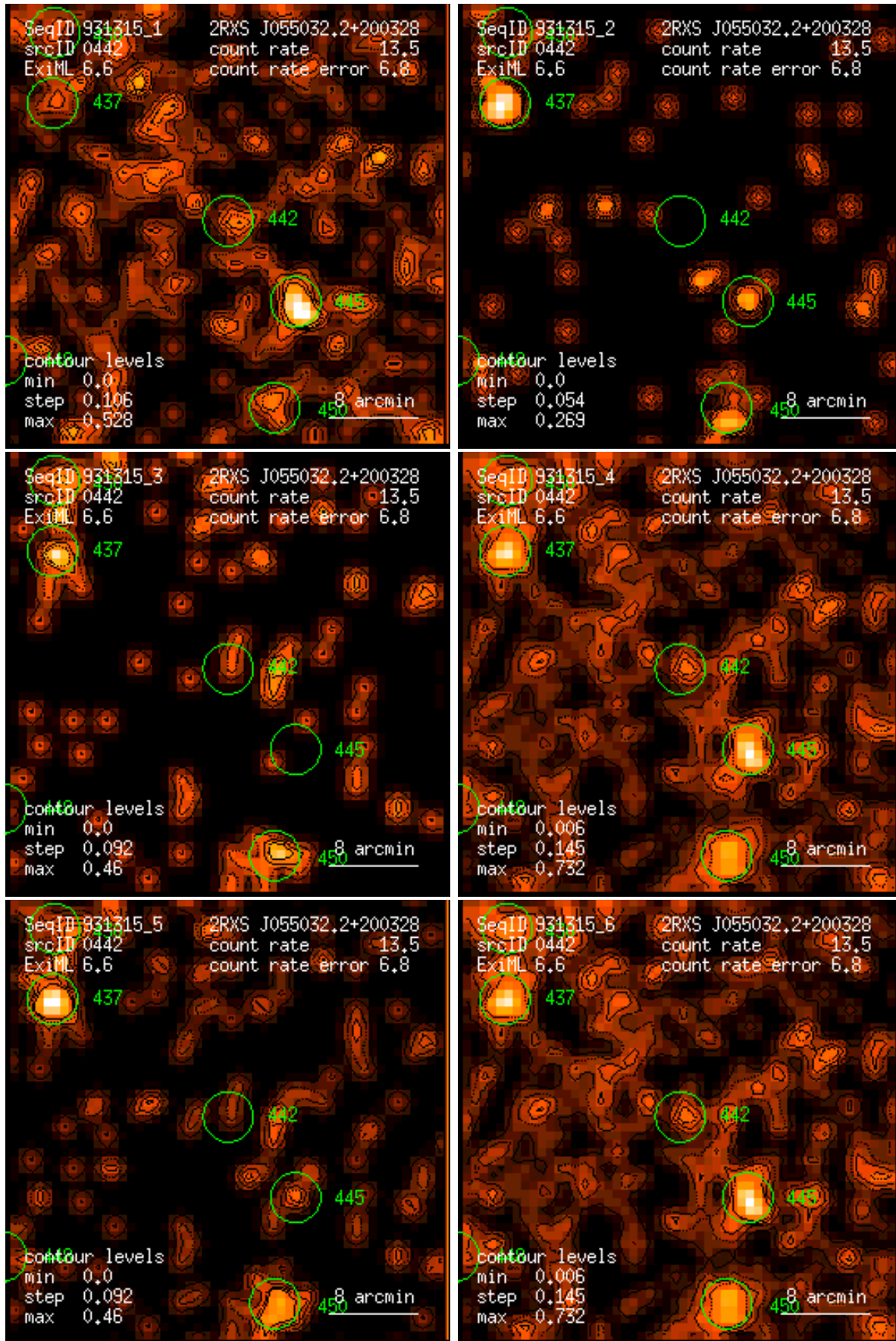
Figure 442: RASS 931315: detection 0442: band rate images, Gaussian filter: (1) PSPC channels 11 – 41, (2) 52 – 90, (3) 91 – 201, (4) 11 – 235, (5) 52 – 201, (6) 11 – 201. Broad band rates in counts/ks. Band rate contour levels in counts/ks/arcmin 2 .
