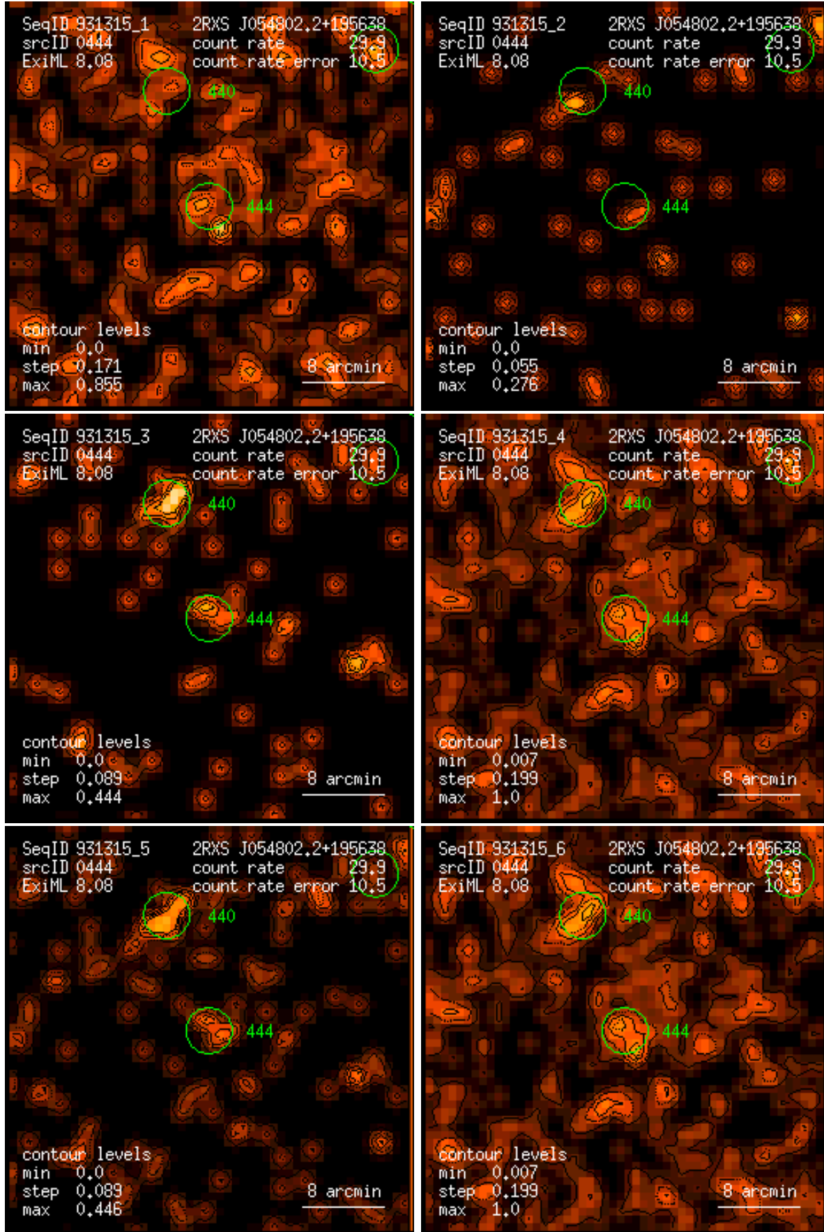
Figure 444: RASS 931315: detection 0444: band rate images, Gaussian filter: (1) PSPC channels 11 – 41, (2) 52 – 90, (3) 91 – 201, (4) 11 – 235, (5) 52 – 201, (6) 11 – 201. Broad band rates in counts/ks. Band rate contour levels in counts/ks/arcmin 2 .
