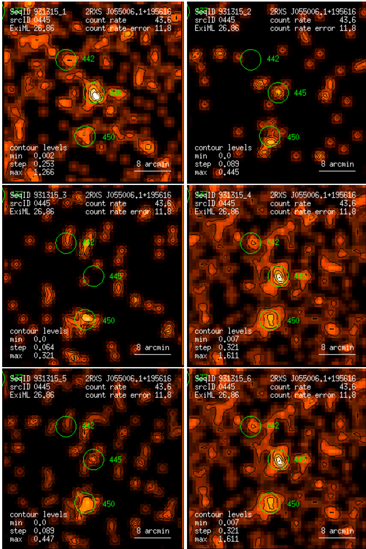
Figure 445: RASS 931315: detection 0445: band rate images, Gaussian filter: (1) PSPC channels 11 – 41, (2) 52 – 90, (3) 91 – 201, (4) 11 – 235, (5) 52 – 201, (6) 11 – 201. Broad band rates in counts/ks. Band rate contour levels in counts/ks/arcmin 2 .
