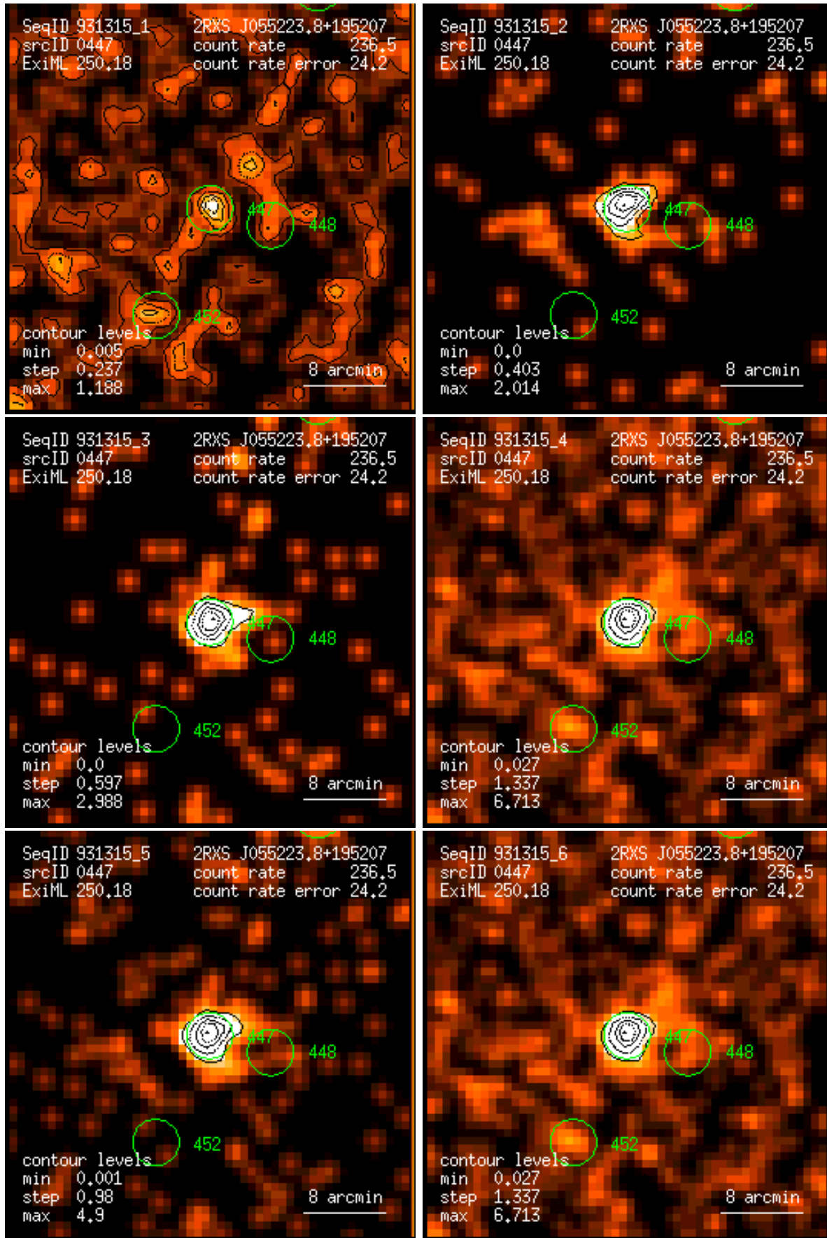
Figure 447: RASS 931315: detection 0447: band rate images, Gaussian filter: (1) PSPC channels 11 – 41, (2) 52 – 90, (3) 91 – 201, (4) 11 – 235, (5) 52 – 201, (6) 11 – 201. Broad band rates in counts/ks. Band rate contour levels in counts/ks/arcmin 2 .
