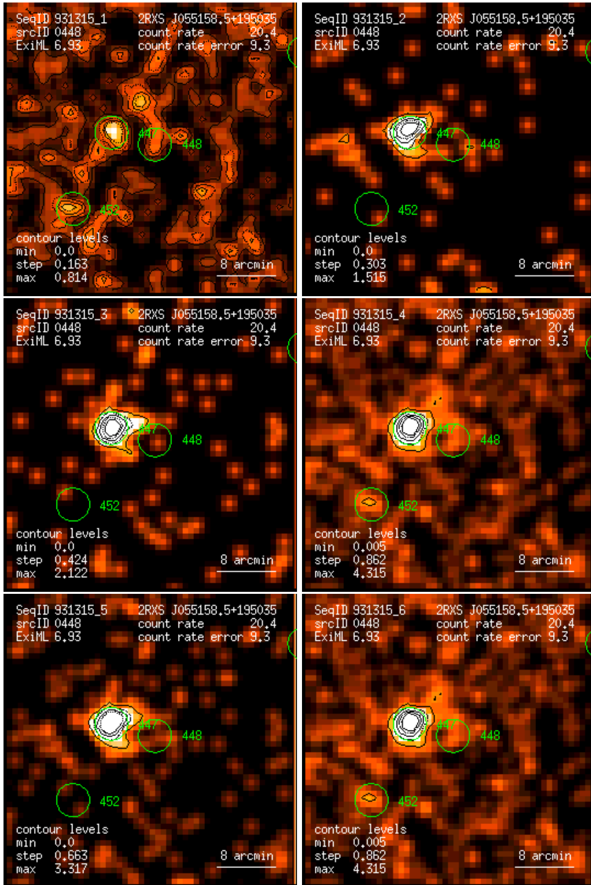
Figure 448: RASS 931315: detection 0448: band rate images, Gaussian filter: (1) PSPC channels 11 – 41, (2) 52 – 90, (3) 91 – 201, (4) 11 – 235, (5) 52 – 201, (6) 11 – 201. Broad band rates in counts/ks. Band rate contour levels in counts/ks/arcmin 2 .
