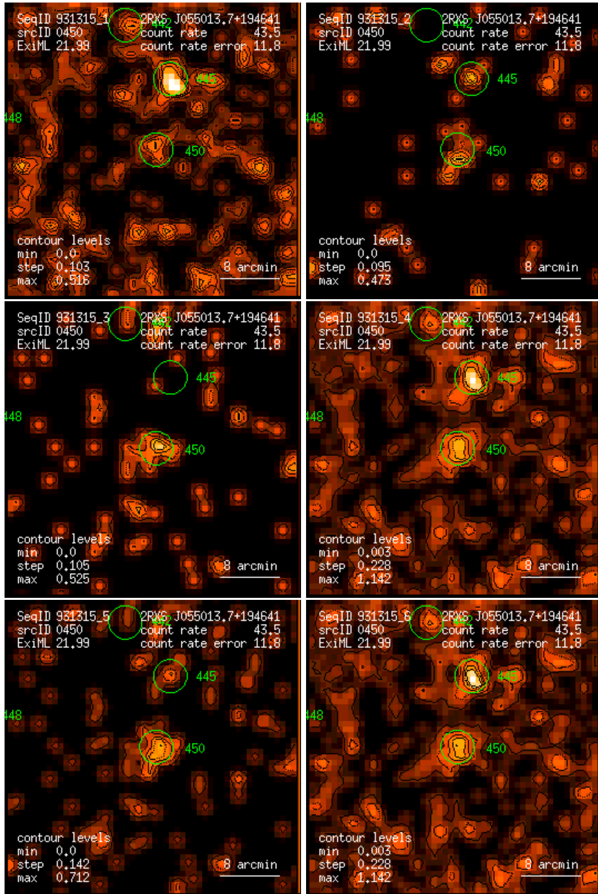
Figure 450: RASS 931315: detection 0450: band rate images, Gaussian filter: (1) PSPC channels 11 – 41, (2) 52 – 90, (3) 91 – 201, (4) 11 – 235, (5) 52 – 201, (6) 11 – 201. Broad band rates in counts/ks. Band rate contour levels in counts/ks/arcmin 2 .
