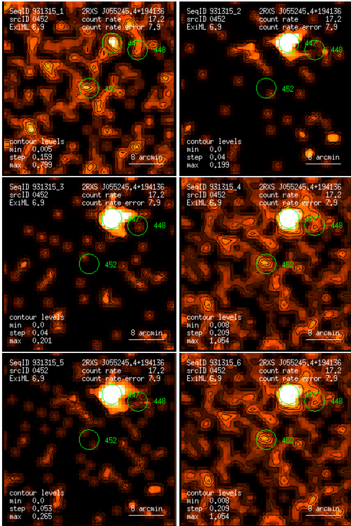
Figure 452: RASS 931315: detection 0452: band rate images, Gaussian filter: (1) PSPC channels 11 – 41, (2) 52 – 90, (3) 91 – 201, (4) 11 – 235, (5) 52 – 201, (6) 11 – 201. Broad band rates in counts/ks. Band rate contour levels in counts/ks/arcmin 2 .
