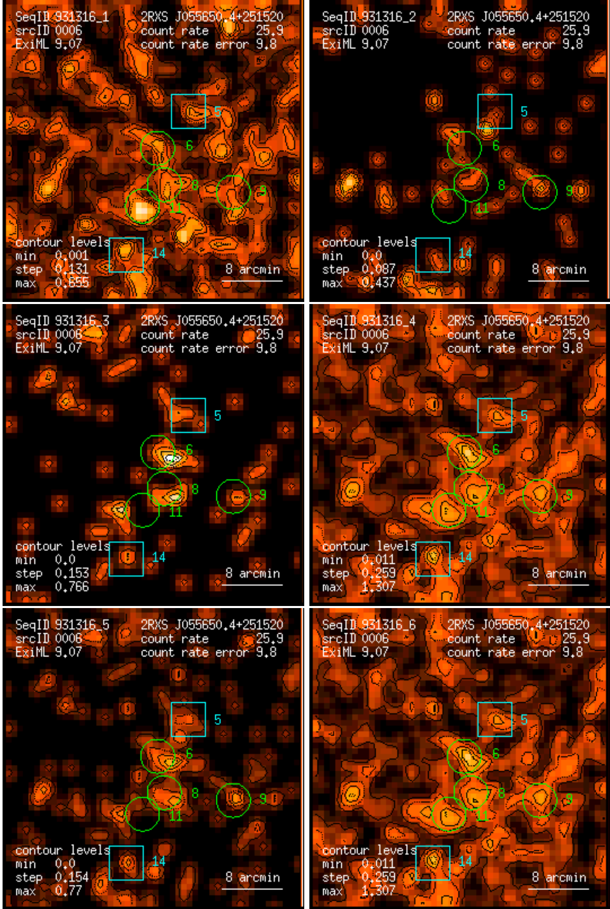
Figure 6: RASS 931316: detection 0006: band rate images, Gaussian filter: (1) PSPC channels 11 – 41, (2) 52 – 90, (3) 91 – 201, (4) 11 – 235, (5) 52 – 201, (6) 11 – 201. Broad band rates in counts/ks. Band rate contour levels in counts/ks/arcmin 2 .
