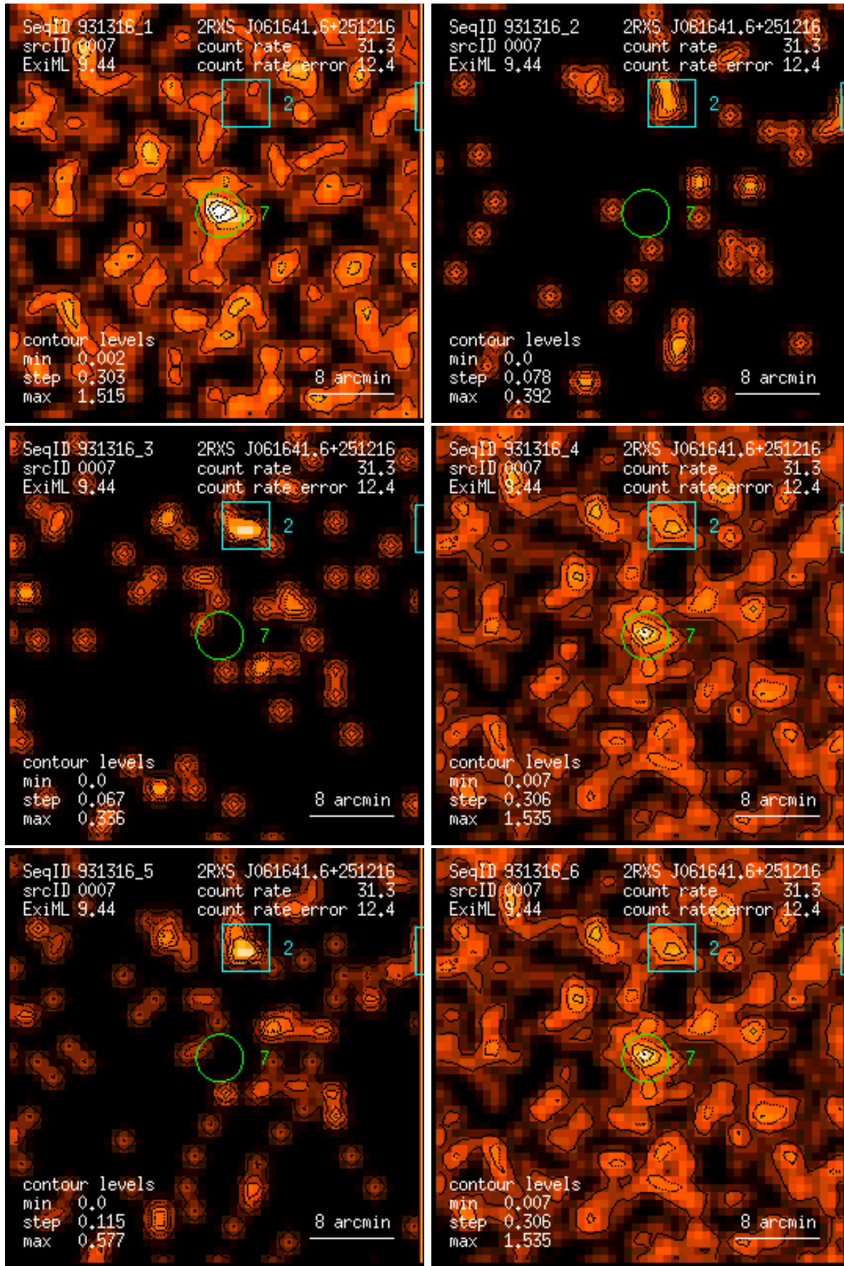
Figure 7: RASS 931316: detection 0007: band rate images, Gaussian filter: (1) PSPC channels 11 – 41, (2) 52 – 90, (3) 91 – 201, (4) 11 – 235, (5) 52 – 201, (6) 11 – 201. Broad band rates in counts/ks. Band rate contour levels in counts/ks/arcmin 2 .
