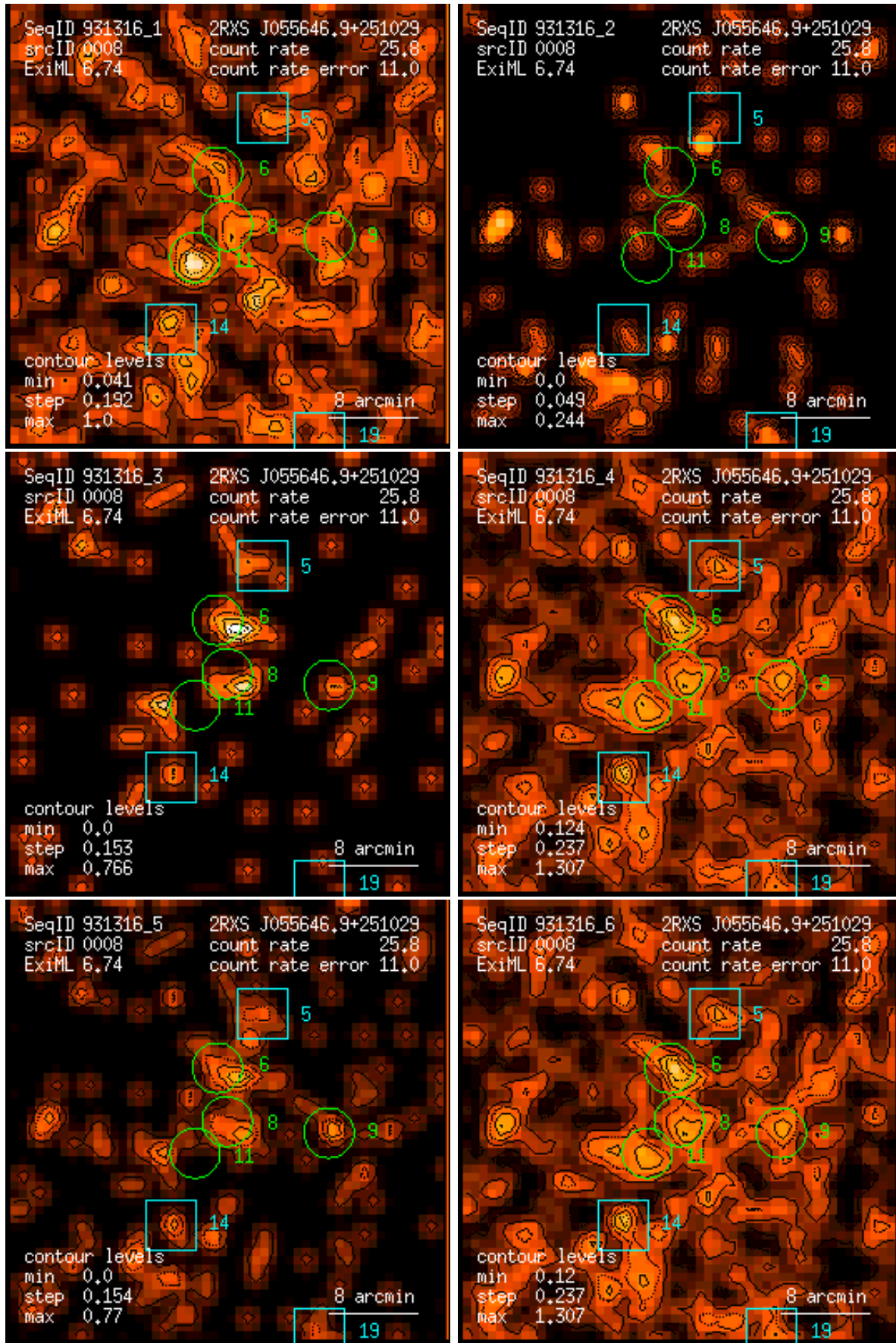
Figure 8: RASS 931316: detection 0008: band rate images, Gaussian filter: (1) PSPC channels 11 – 41, (2) 52 – 90, (3) 91 – 201, (4) 11 – 235, (5) 52 – 201, (6) 11 – 201. Broad band rates in counts/ks. Band rate contour levels in counts/ks/arcmin 2 .
