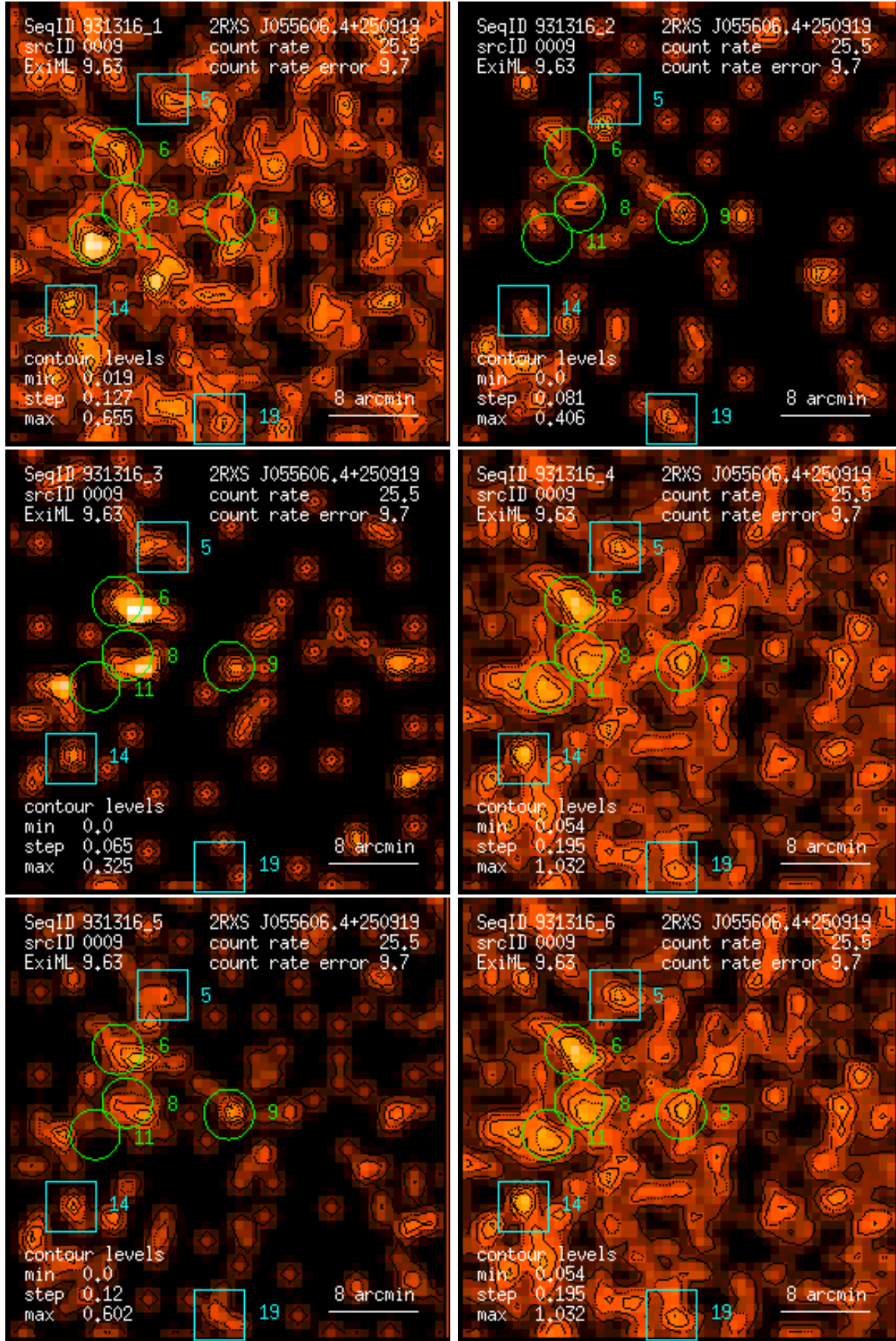
Figure 9: RASS 931316: detection 0009: band rate images, Gaussian filter: (1) PSPC channels 11 – 41, (2) 52 – 90, (3) 91 – 201, (4) 11 – 235, (5) 52 – 201, (6) 11 – 201. Broad band rates in counts/ks. Band rate contour levels in counts/ks/arcmin 2 .
