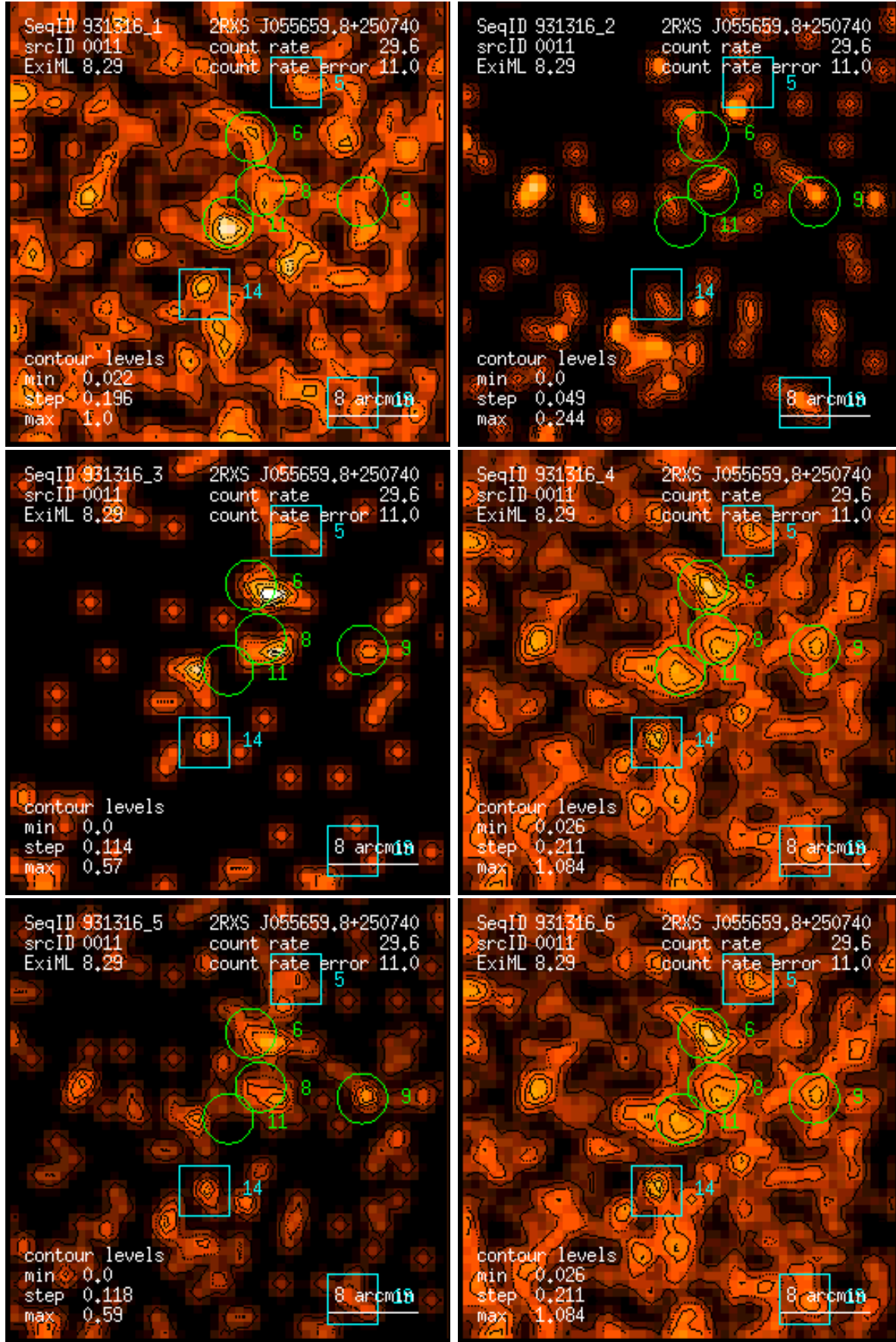
Figure 11: RASS 931316: detection 0011: band rate images, Gaussian filter: (1) PSPC channels 11 – 41, (2) 52 – 90, (3) 91 – 201, (4) 11 – 235, (5) 52 – 201, (6) 11 – 201. Broad band rates in counts/ks. Band rate contour levels in counts/ks/arcmin 2 .
