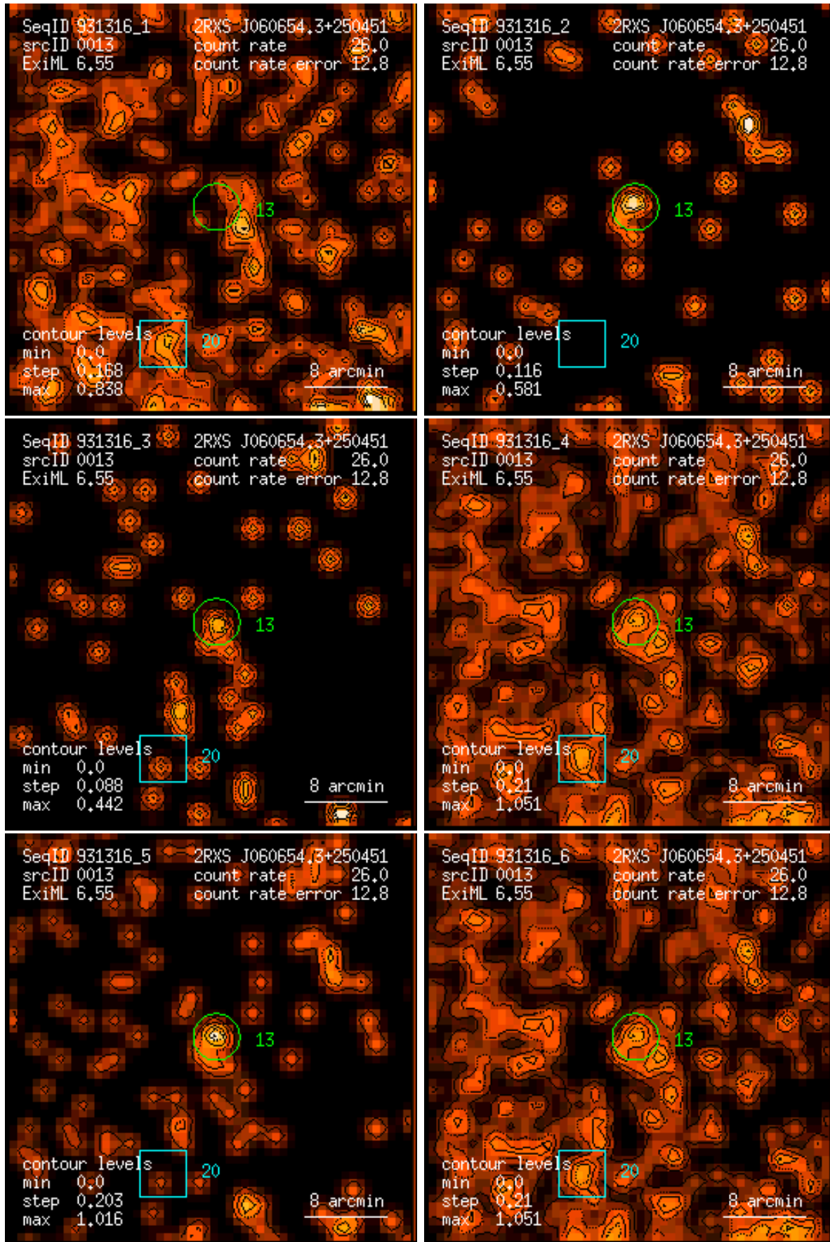
Figure 13: RASS 931316: detection 0013: band rate images, Gaussian filter: (1) PSPC channels 11 – 41, (2) 52 – 90, (3) 91 – 201, (4) 11 – 235, (5) 52 – 201, (6) 11 – 201. Broad band rates in counts/ks. Band rate contour levels in counts/ks/arcmin 2 .
