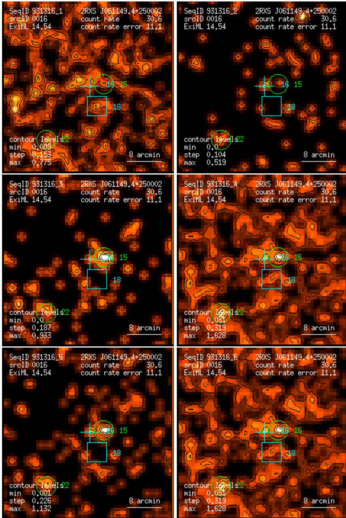
Figure 16: RASS 931316: detection 0016: band rate images, Gaussian filter: (1) PSPC channels 11 – 41, (2) 52 – 90, (3) 91 – 201, (4) 11 – 235, (5) 52 – 201, (6) 11 – 201. Broad band rates in counts/ks. Band rate contour levels in counts/ks/arcmin 2 .
