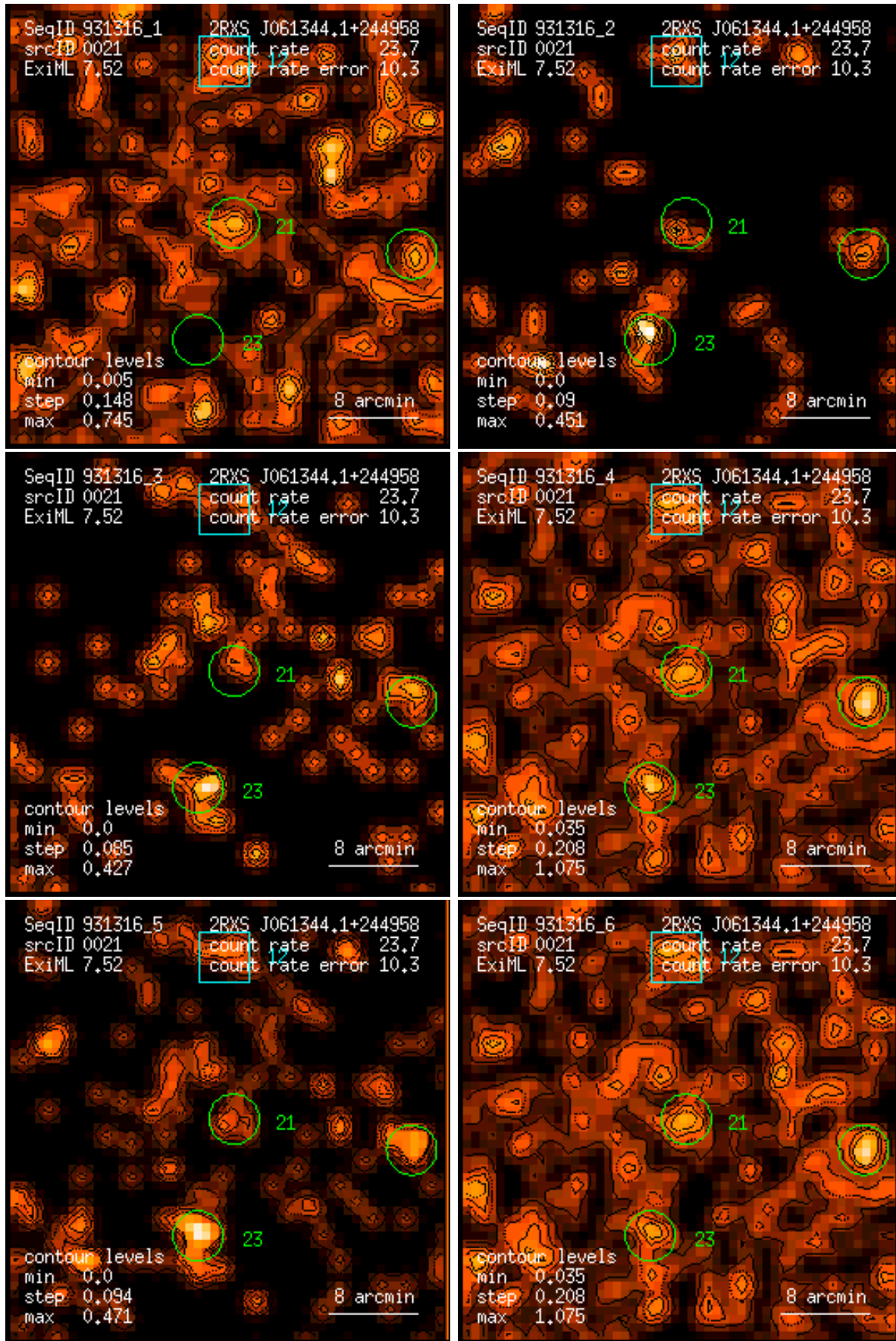
Figure 21: RASS 931316: detection 0021: band rate images, Gaussian filter: (1) PSPC channels 11 – 41, (2) 52 – 90, (3) 91 – 201, (4) 11 – 235, (5) 52 – 201, (6) 11 – 201. Broad band rates in counts/ks. Band rate contour levels in counts/ks/arcmin 2 .
