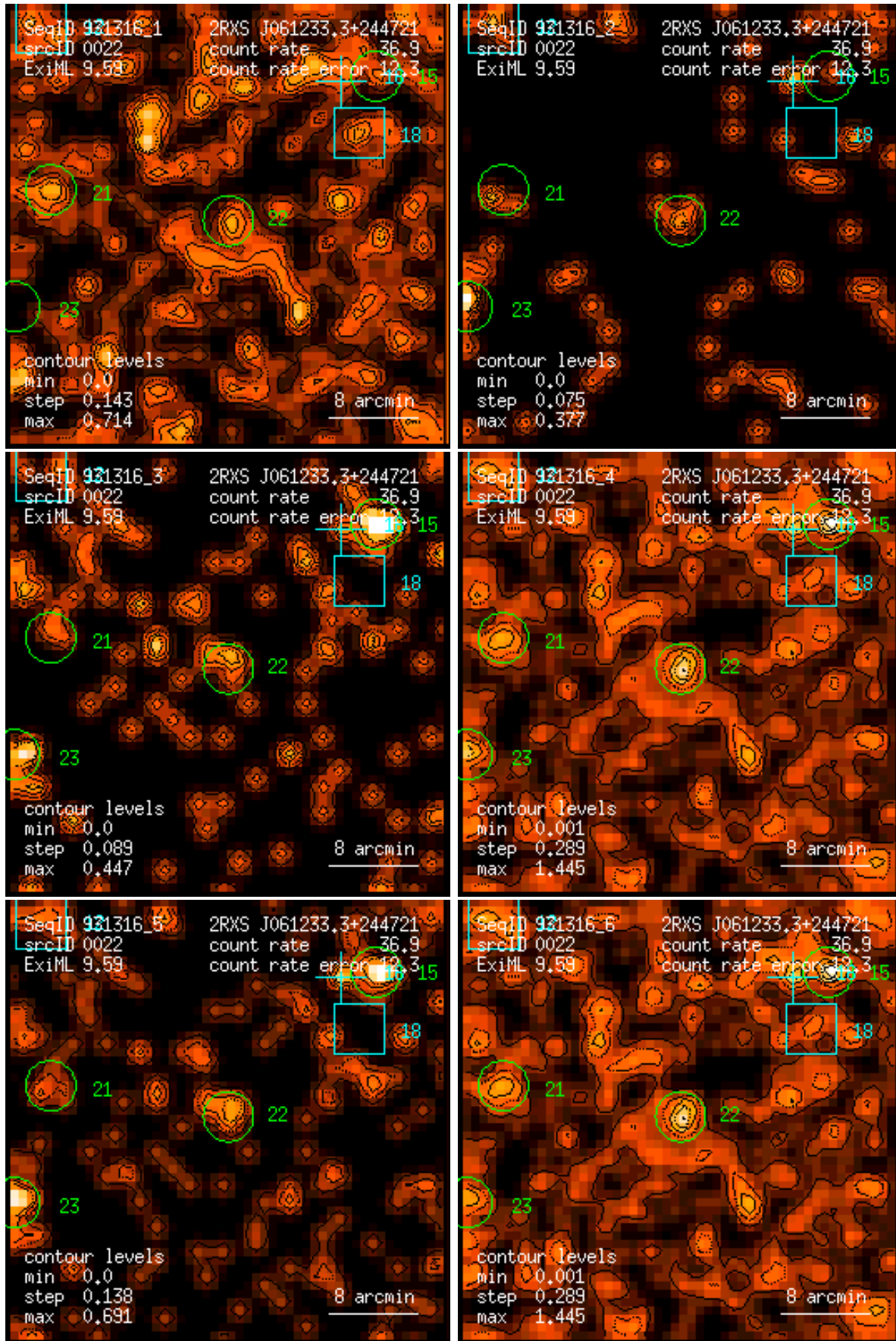
Figure 22: RASS 931316: detection 0022: band rate images, Gaussian filter: (1) PSPC channels 11 – 41, (2) 52 – 90, (3) 91 – 201, (4) 11 – 235, (5) 52 – 201, (6) 11 – 201. Broad band rates in counts/ks. Band rate contour levels in counts/ks/arcmin 2 .
