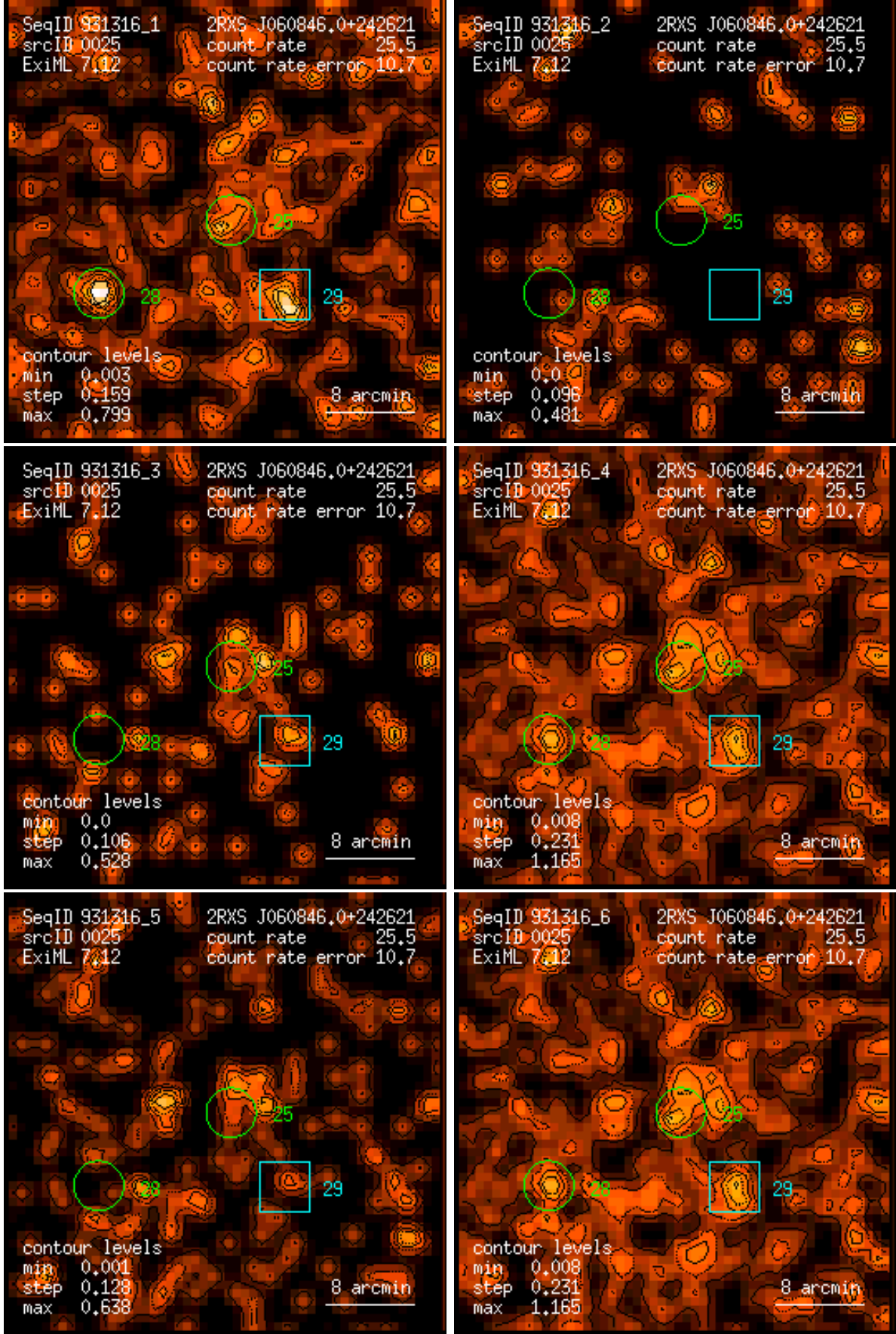
Figure 25: RASS 931316: detection 0025: band rate images, Gaussian filter: (1) PSPC channels 11 – 41, (2) 52 – 90, (3) 91 – 201, (4) 11 – 235, (5) 52 – 201, (6) 11 – 201. Broad band rates in counts/ks. Band rate contour levels in counts/ks/arcmin 2 .
