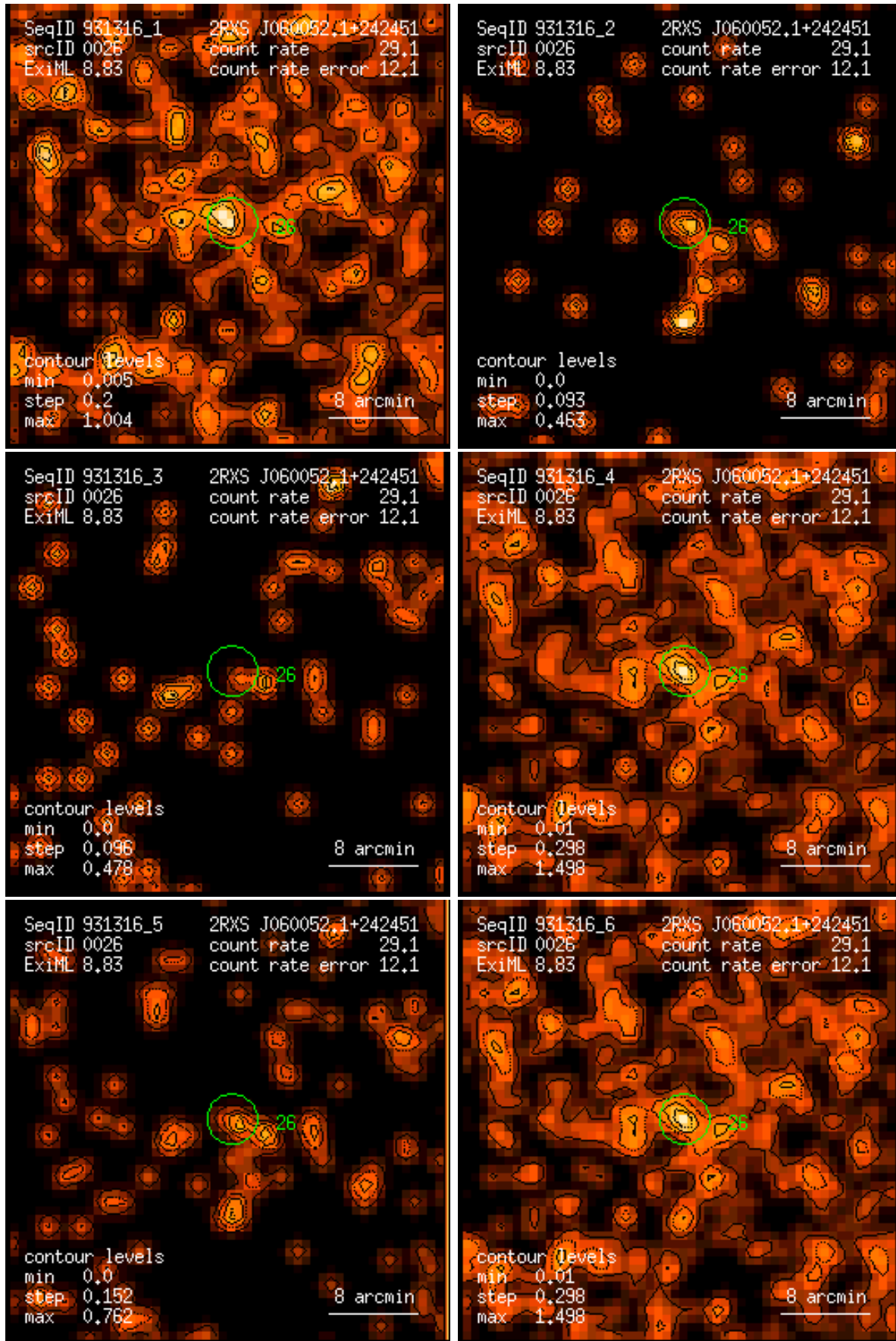
Figure 26: RASS 931316: detection 0026: band rate images, Gaussian filter: (1) PSPC channels 11 – 41, (2) 52 – 90, (3) 91 – 201, (4) 11 – 235, (5) 52 – 201, (6) 11 – 201. Broad band rates in counts/ks. Band rate contour levels in counts/ks/arcmin 2 .
