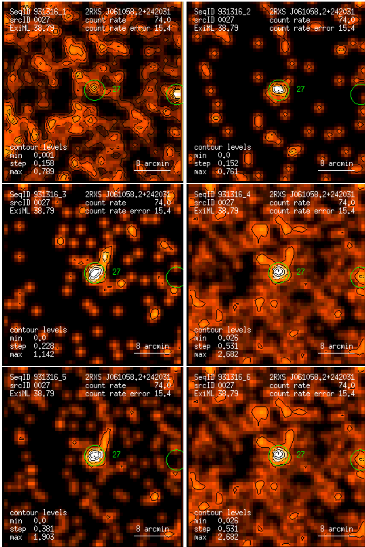
Figure 27: RASS 931316: detection 0027: band rate images, Gaussian filter: (1) PSPC channels 11 – 41, (2) 52 – 90, (3) 91 – 201, (4) 11 – 235, (5) 52 – 201, (6) 11 – 201. Broad band rates in counts/ks. Band rate contour levels in counts/ks/arcmin 2 .
