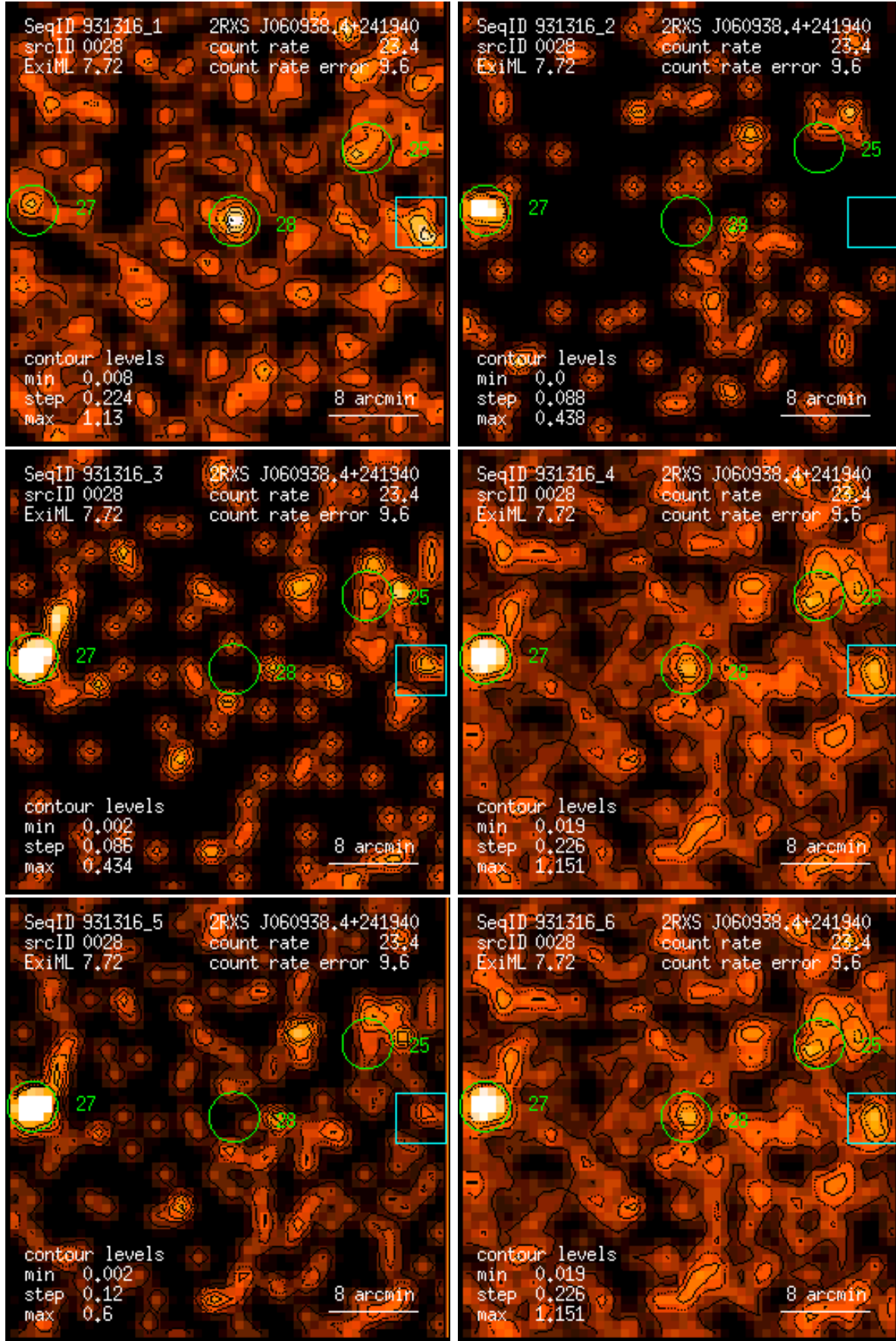
Figure 28: RASS 931316: detection 0028: band rate images, Gaussian filter: (1) PSPC channels 11 – 41, (2) 52 – 90, (3) 91 – 201, (4) 11 – 235, (5) 52 – 201, (6) 11 – 201. Broad band rates in counts/ks. Band rate contour levels in counts/ks/arcmin 2 .
