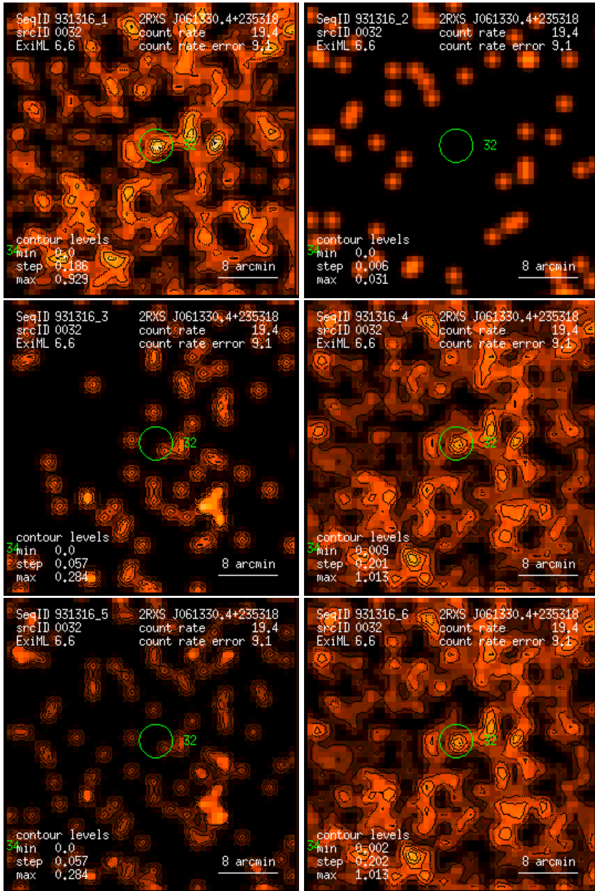
Figure 32: RASS 931316: detection 0032: band rate images, Gaussian filter: (1) PSPC channels 11 – 41, (2) 52 – 90, (3) 91 – 201, (4) 11 – 235, (5) 52 – 201, (6) 11 – 201. Broad band rates in counts/ks. Band rate contour levels in counts/ks/arcmin 2 .
