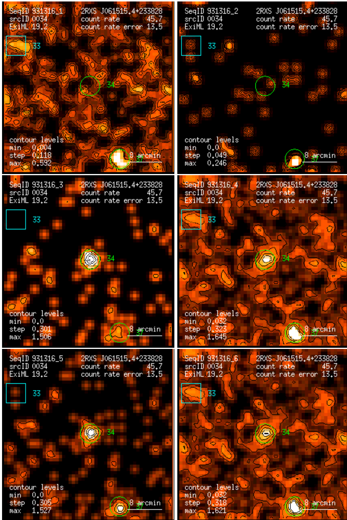
Figure 34: RASS 931316: detection 0034: band rate images, Gaussian filter: (1) PSPC channels 11 – 41, (2) 52 – 90, (3) 91 – 201, (4) 11 – 235, (5) 52 – 201, (6) 11 – 201. Broad band rates in counts/ks. Band rate contour levels in counts/ks/arcmin 2 .
