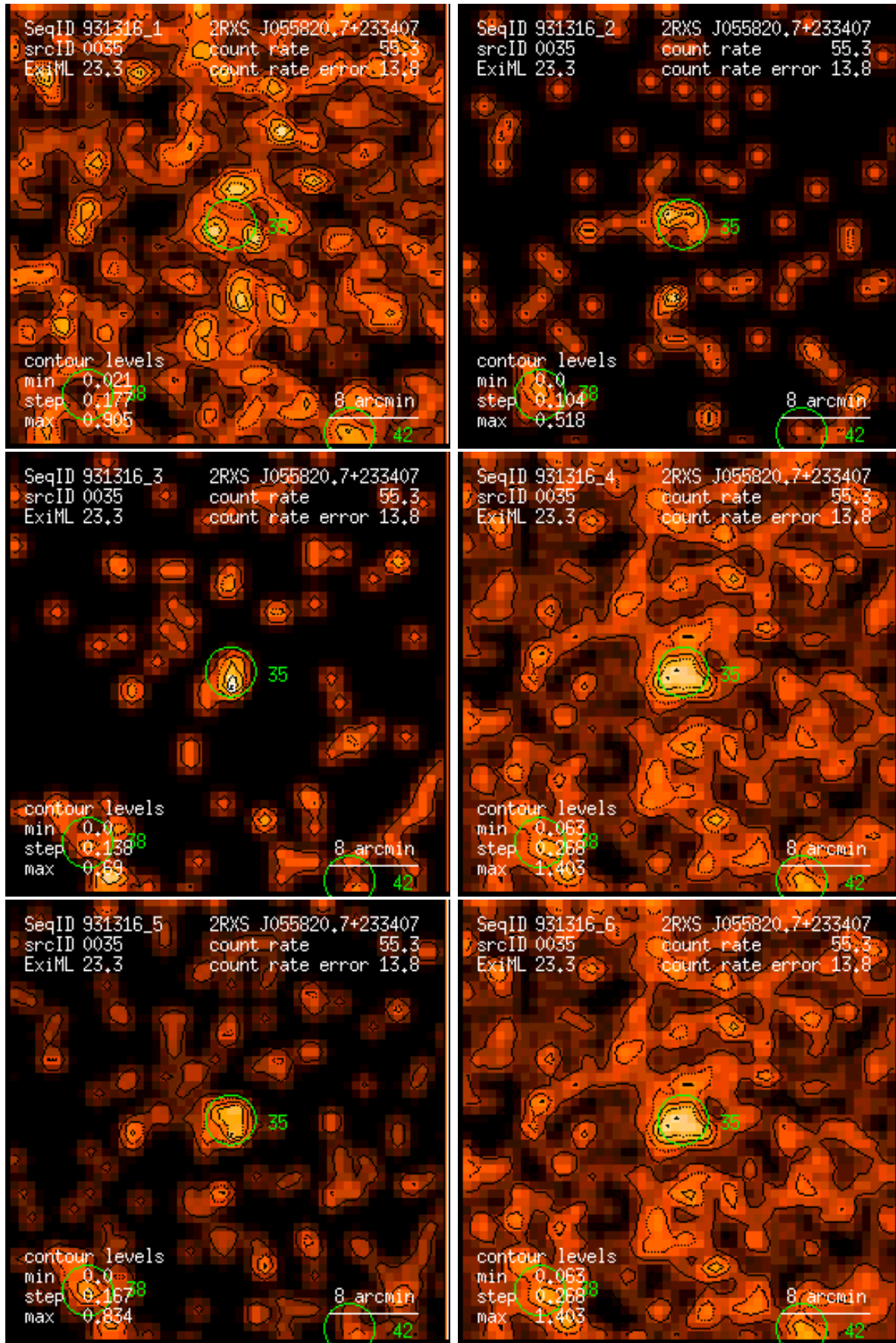
Figure 35: RASS 931316: detection 0035: band rate images, Gaussian filter: (1) PSPC channels 11 – 41, (2) 52 – 90, (3) 91 – 201, (4) 11 – 235, (5) 52 – 201, (6) 11 – 201. Broad band rates in counts/ks. Band rate contour levels in counts/ks/arcmin 2 .
