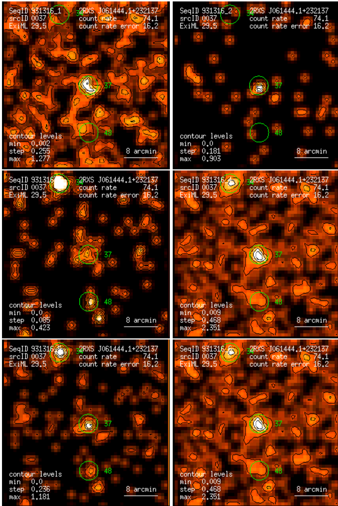
Figure 37: RASS 931316: detection 0037: band rate images, Gaussian filter: (1) PSPC channels 11 – 41, (2) 52 – 90, (3) 91 – 201, (4) 11 – 235, (5) 52 – 201, (6) 11 – 201. Broad band rates in counts/ks. Band rate contour levels in counts/ks/arcmin 2 .
