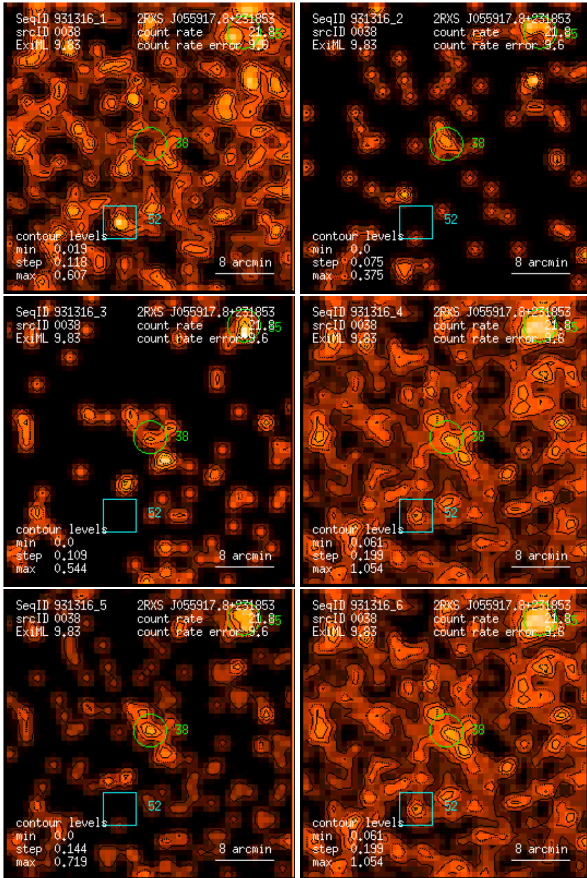
Figure 38: RASS 931316: detection 0038: band rate images, Gaussian filter: (1) PSPC channels 11 – 41, (2) 52 – 90, (3) 91 – 201, (4) 11 – 235, (5) 52 – 201, (6) 11 – 201. Broad band rates in counts/ks. Band rate contour levels in counts/ks/arcmin 2 .
