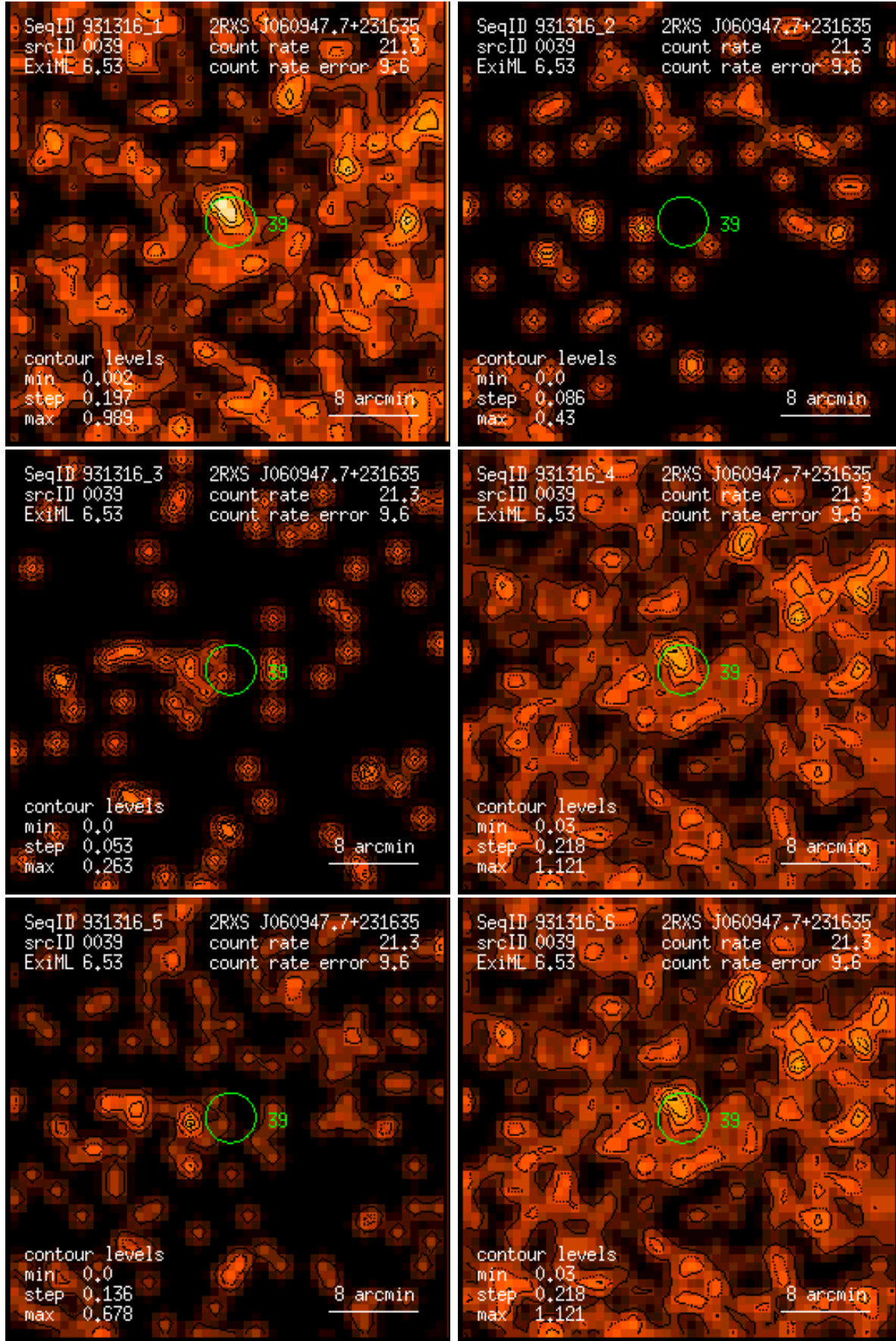
Figure 39: RASS 931316: detection 0039: band rate images, Gaussian filter: (1) PSPC channels 11 – 41, (2) 52 – 90, (3) 91 – 201, (4) 11 – 235, (5) 52 – 201, (6) 11 – 201. Broad band rates in counts/ks. Band rate contour levels in counts/ks/arcmin 2 .
