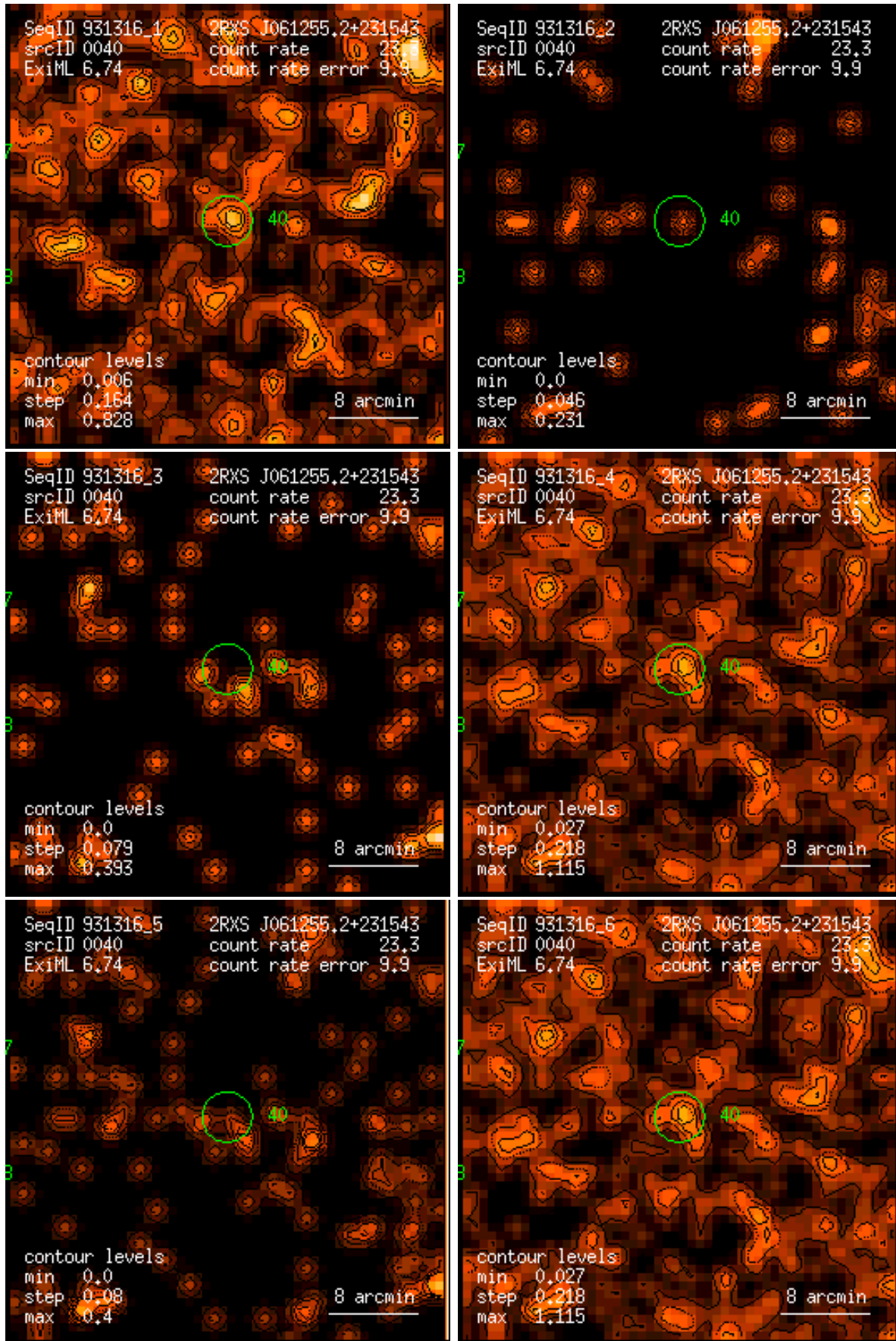
Figure 40: RASS 931316: detection 0040: band rate images, Gaussian filter: (1) PSPC channels 11 – 41, (2) 52 – 90, (3) 91 – 201, (4) 11 – 235, (5) 52 – 201, (6) 11 – 201. Broad band rates in counts/ks. Band rate contour levels in counts/ks/arcmin 2 .
