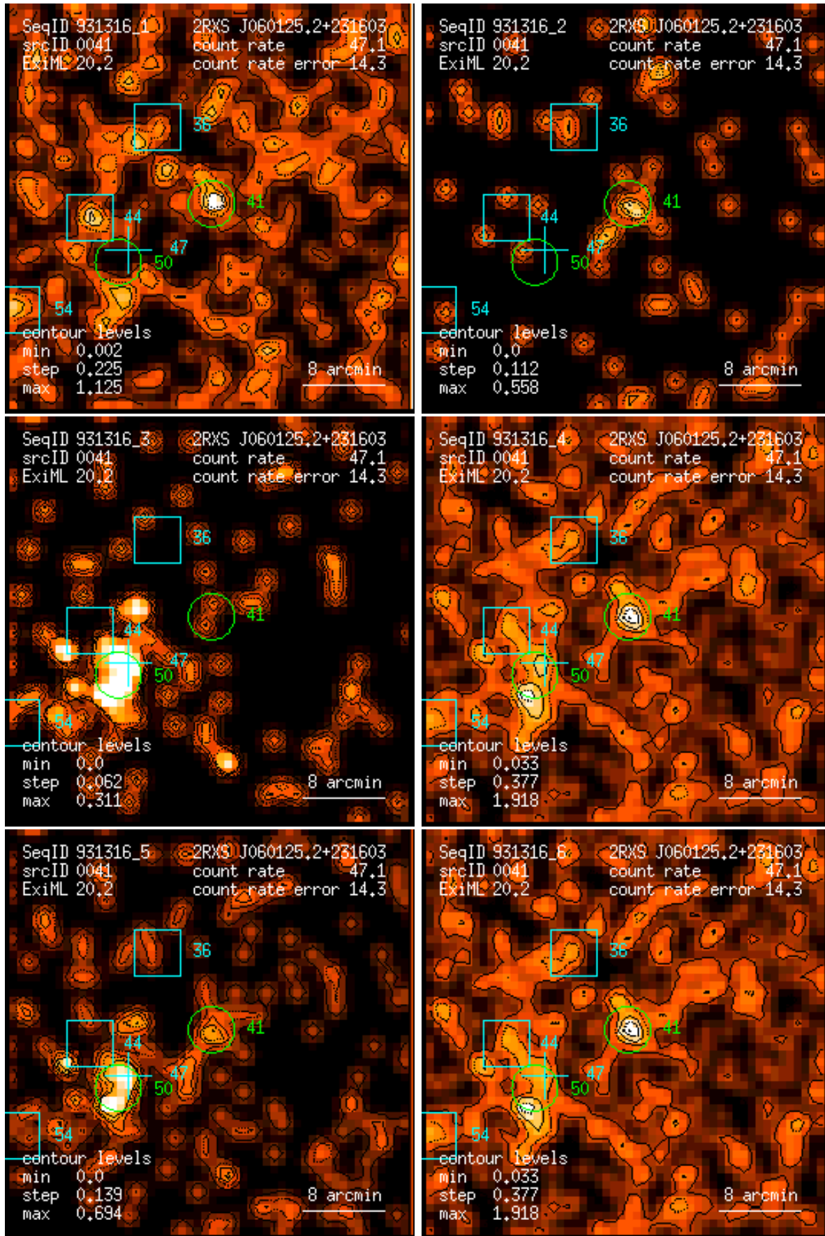
Figure 41: RASS 931316: detection 0041: band rate images, Gaussian filter: (1) PSPC channels 11 – 41, (2) 52 – 90, (3) 91 – 201, (4) 11 – 235, (5) 52 – 201, (6) 11 – 201. Broad band rates in counts/ks. Band rate contour levels in counts/ks/arcmin 2 .
