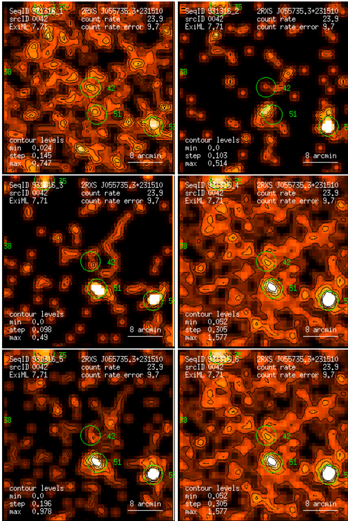
Figure 42: RASS 931316: detection 0042: band rate images, Gaussian filter: (1) PSPC channels 11 – 41, (2) 52 – 90, (3) 91 – 201, (4) 11 – 235, (5) 52 – 201, (6) 11 – 201. Broad band rates in counts/ks. Band rate contour levels in counts/ks/arcmin 2 .
